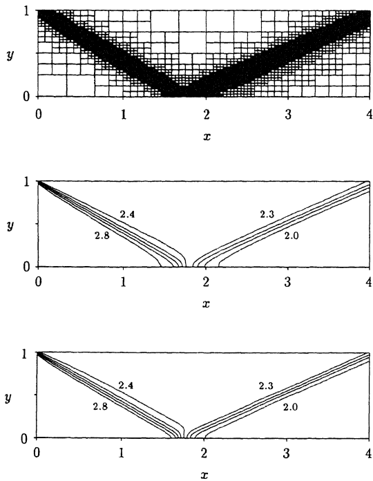
Figure 3: Grid and iso-lines of the Mach number for the shock reflection problem on a locally refined grid; second-order discretisation; L = 5 .
