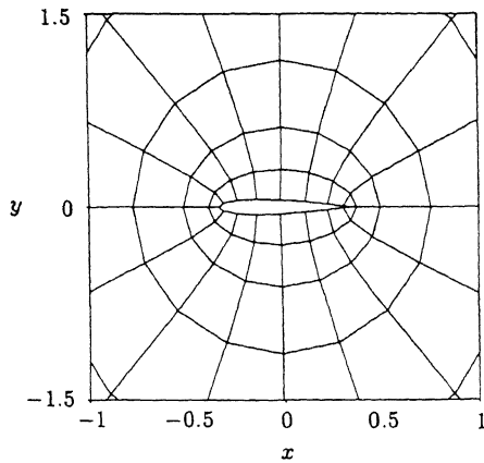
Figure 5: Uniform grid of level l = 1 , around NACA0012 airfoil.
