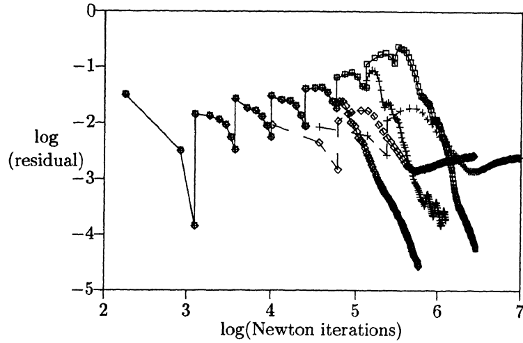
Figure 4: Residual versus amount of work: convergence histories for defect correction and second-order discretisation on uniform and locally refined grids; \diamond : L = 4 ; + : L = 5 ; \square : L = 6 ; —: locally refined; — —: uniform.
