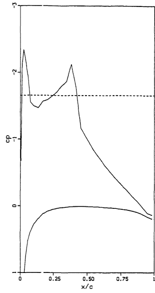
Lower airfoil.
