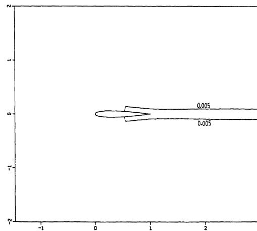
Fig. 5: Solution NACA0012-airfoil at M_\infty = 0.81 , \alpha = 0^\circ (problem 2.4).
