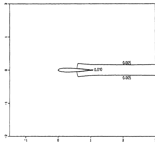
Fig. 6: Solution NACA0012-airfoil at M_\infty = 0.82 , \alpha = 0^\circ (problem 2.5).
