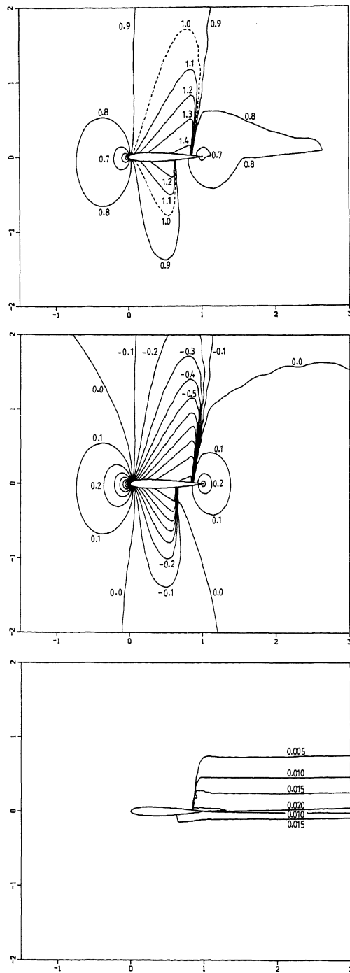
Fig. 4: Solution NACA0012-airfoil at M_\infty = 0.85 , \alpha = 1^\circ (problem 2.3).
