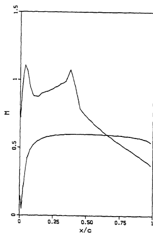
Lower airfoil.
