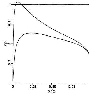
b. Pressure distributions.
