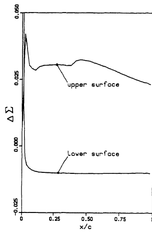
Lower airfoil.
