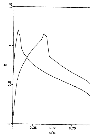
Upper airfoil.
