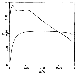
Lower airfoil.
