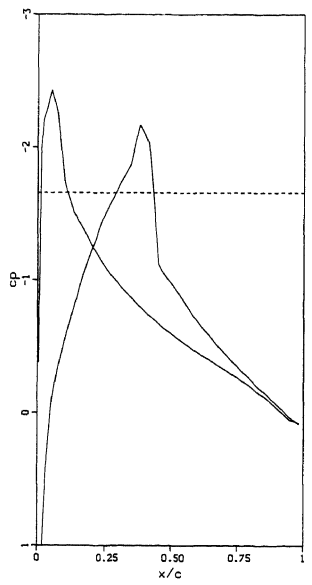
Upper airfoil.
