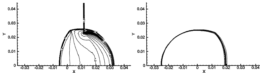
Figure 5. Shock hitting helium bubble, pressure (left) and volume fraction (right) at t = 10.74 \times 10^{-3} .
