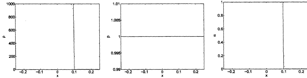
Figure 2. 1D contact discontinuity. p = 1 , u = 1 , \rho_L = 1000 , \rho_R = 1 , \gamma_L = 1.4 and \gamma_R = 1.6 . The grid has 200 cells, 80 time steps and \Delta t/\Delta x = 0.5 (CFL = 0.5). Solid lines: exact solution.
