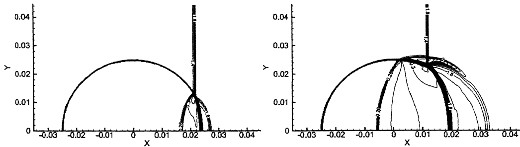
Figure 4. Shock hitting helium bubble, density at t = 2.74 \times 10^{-3} and t = 10.74 \times 10^{-3} .
