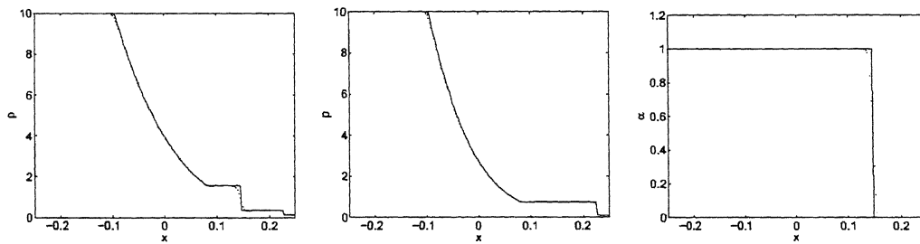
Figure 3. High-pressure, two-fluid Sod problem. (\rho, u, p)_L = (10, 0, 10) , (\rho, u, p)_R = (0.125, 0, 0.1) , \gamma_L = 1.4 and \gamma_R = 1.6 . The grid has 200 cells, 160 time steps, \Delta t/\Delta x = 0.2 (CFL = 0.56). Solid lines: exact solution.
