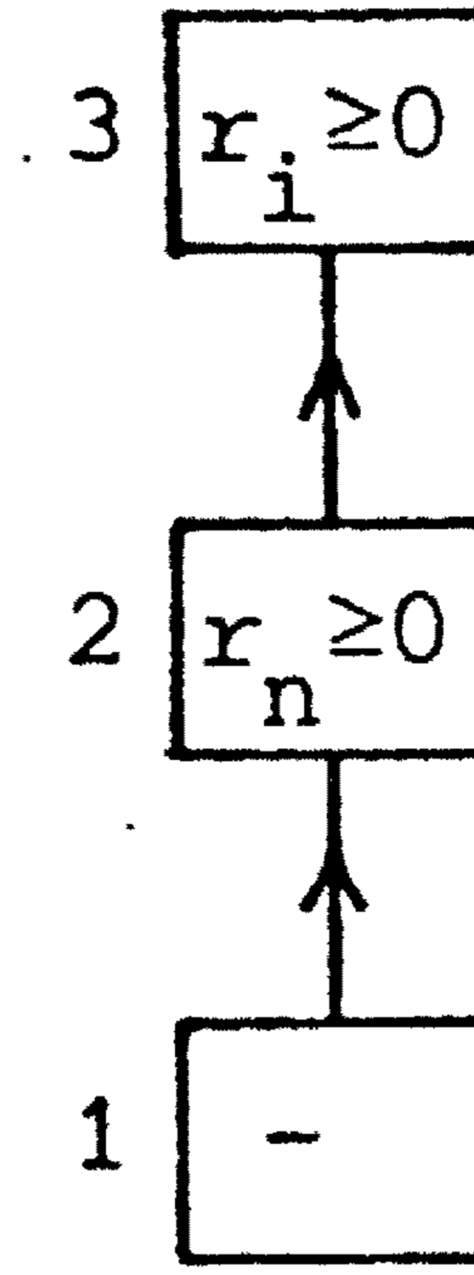
Figure 4 The graph G_4 .
