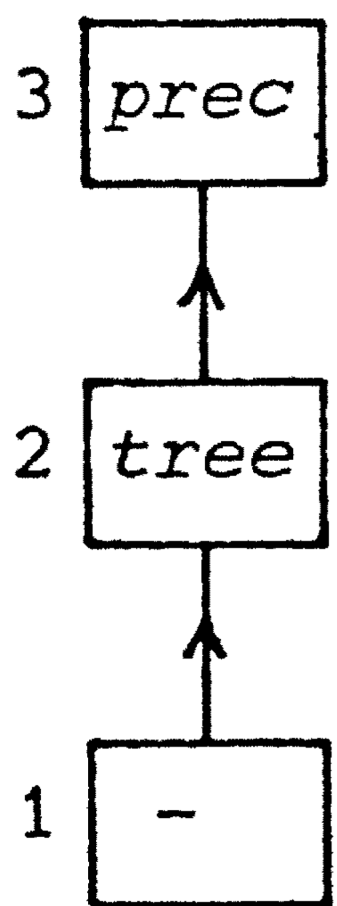
Figure 2 The graph G_2 .
