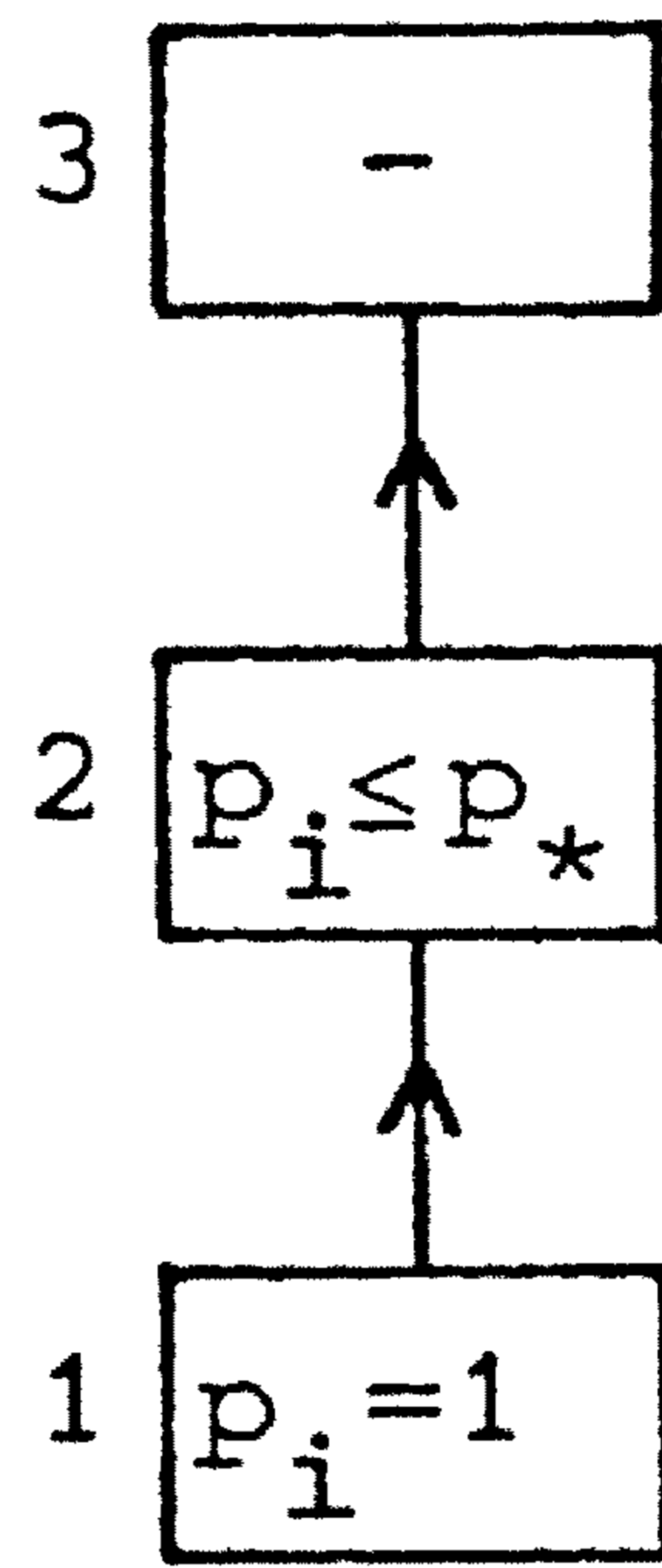
Figure 3 The graph G_3 .
