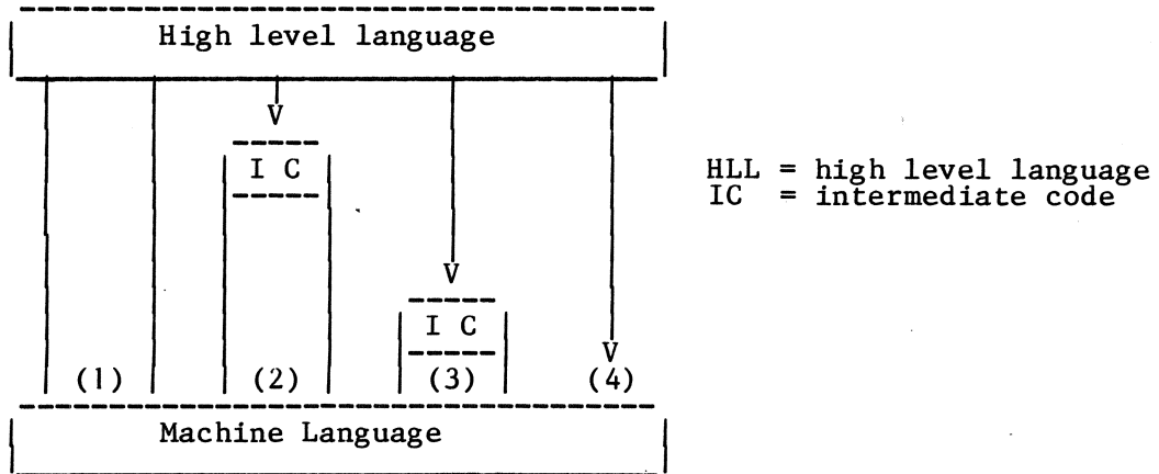
Figure 1. Four types of high level language implementations.
