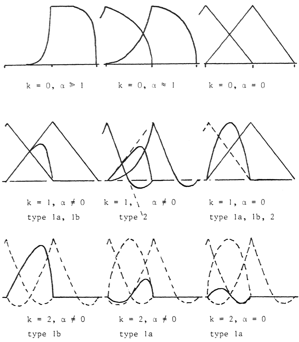
Fig. 2. Several basis functions in E_k^h, k = 0, 1, 2.
