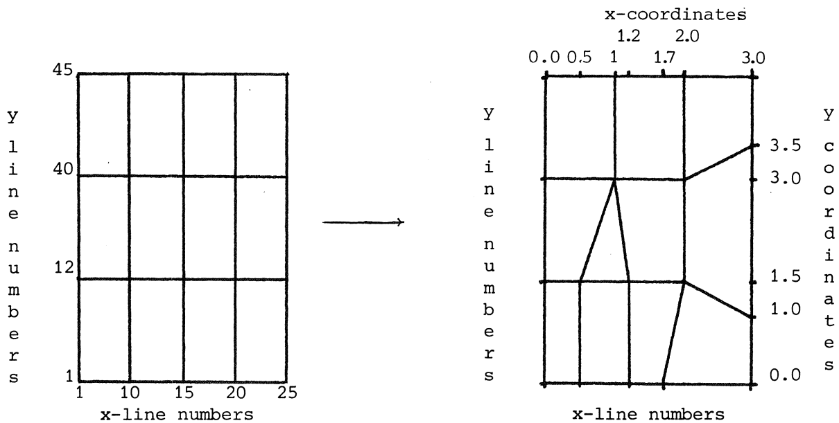
FIGURE 1. The mesh is specified in the SEMMY2 input language by: x(1) = 0, x(10) = 2 * .5, 2 * 1, x(15) = 2 * 1.2, 2 * 1, x(20) = 1.7, 3 * 2, x(25) = 3, y(1) = 0, y(12) = 4 * 1.5, 1, y(40) = 4 * 3., 3.5, y(45) = 4.5.
