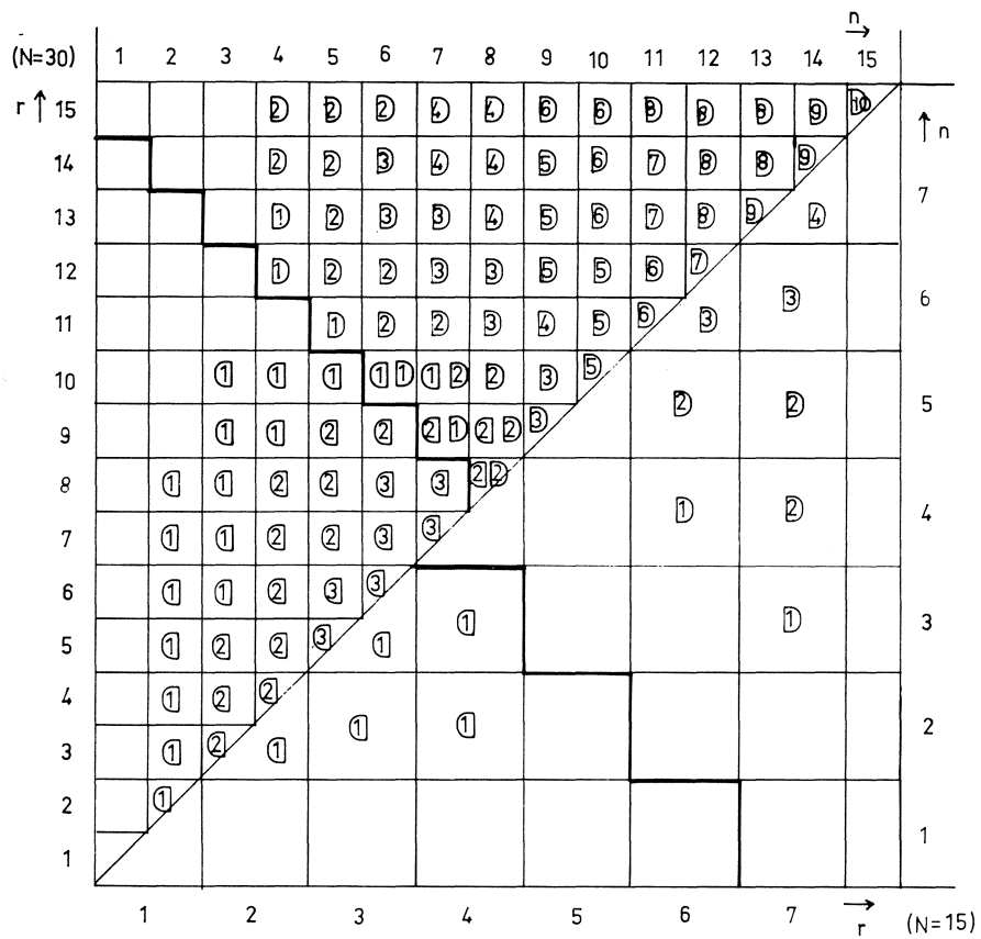
Fig. 2: \square : normal approx. better \square : \chi^2 approx. better N = 15, 30
