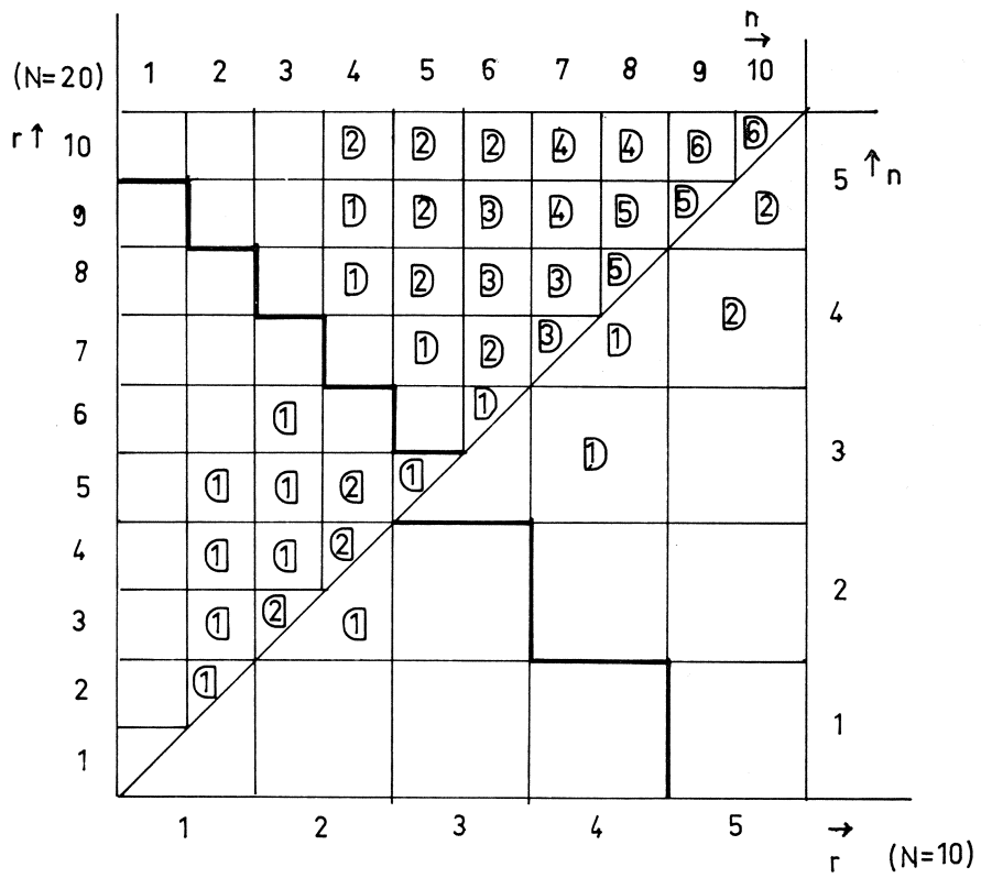
Fig. 1. \circ : normal approx. better \text{D} : \chi^2 approx. better N = 10, 20
