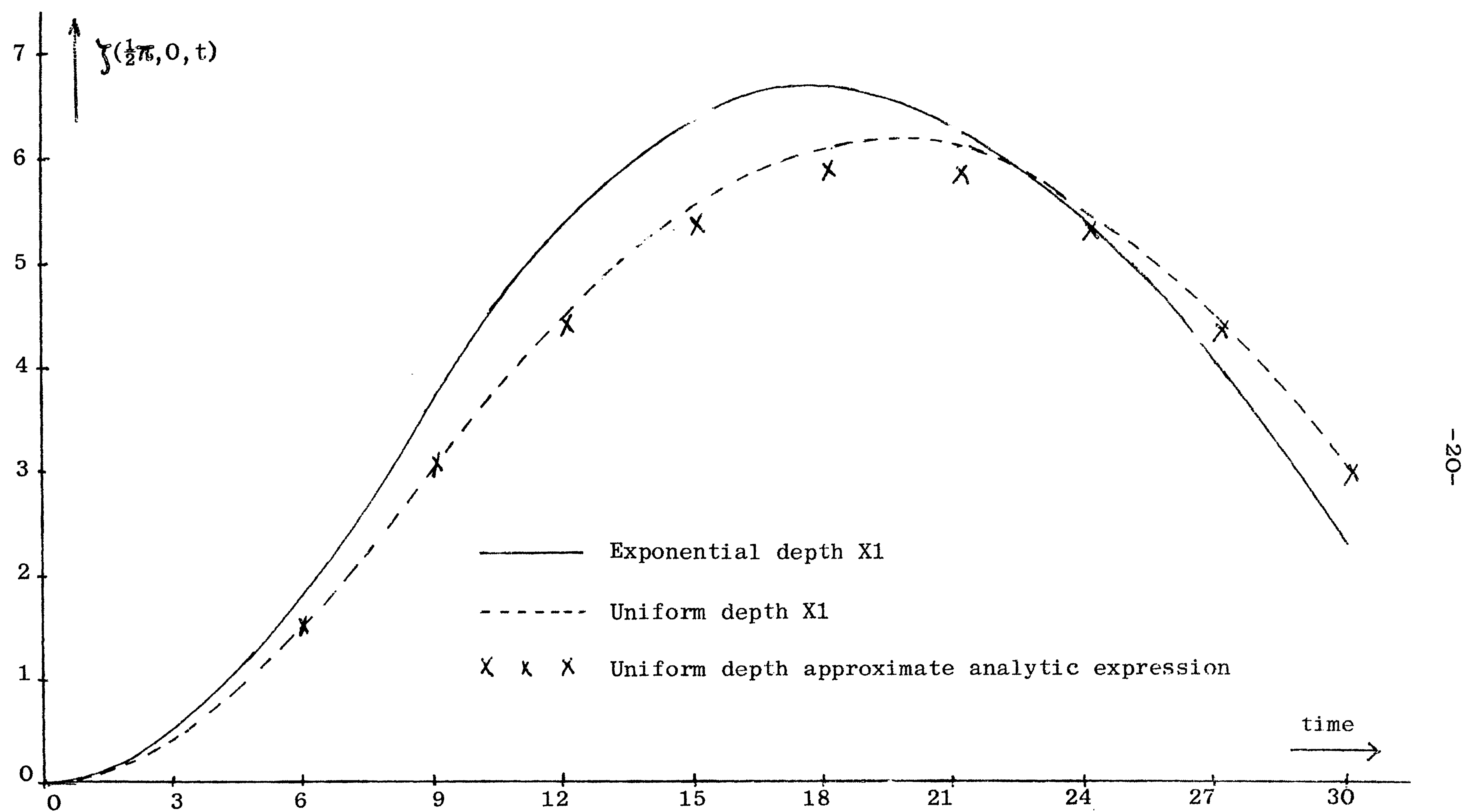
fig.2. Elevation at (\frac{1}{2}\pi, 0) . Windfield U=0 , V=-\sin 0.1t
