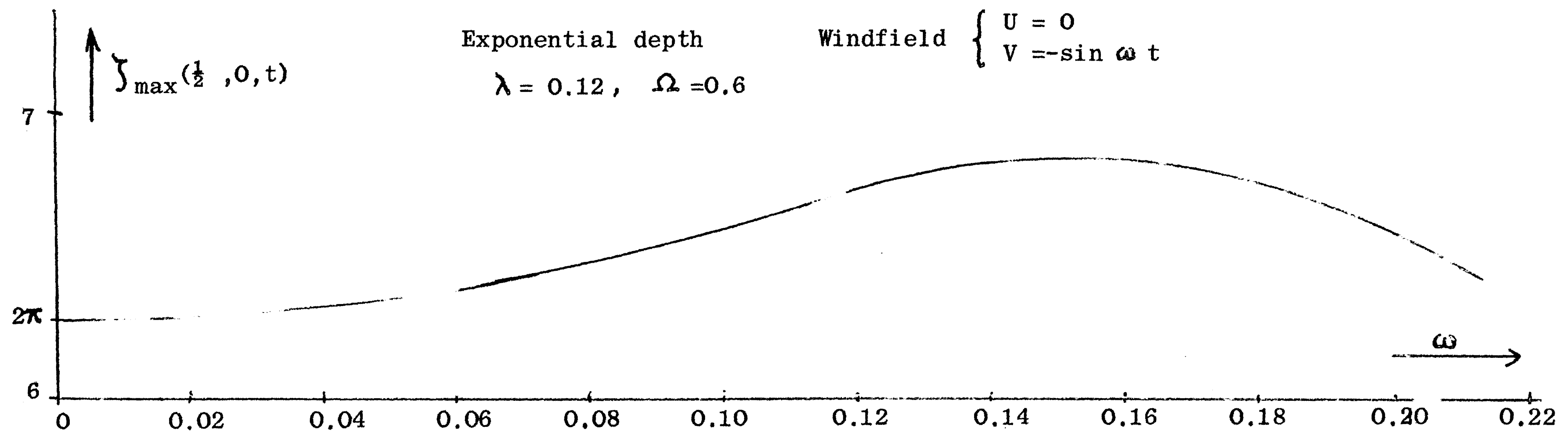
fig.7. Influence of \omega on maximal elevation at (\frac{1}{2}\pi, 0)
