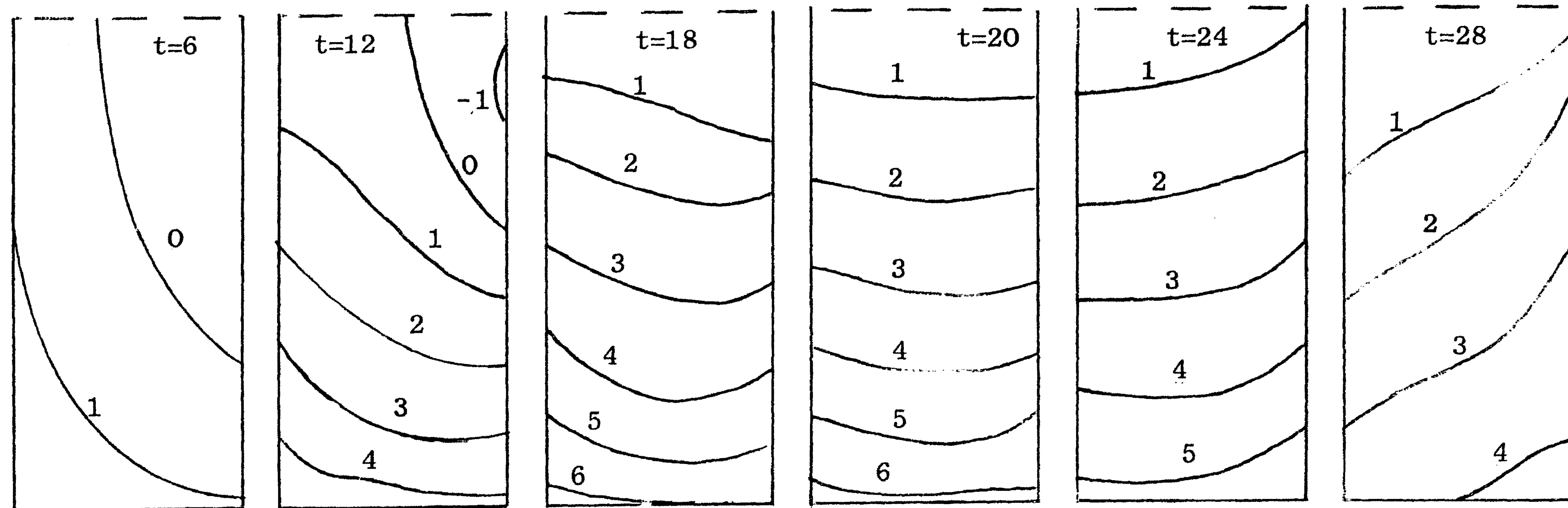
fig.3. Uniform depth. Isohypes due to the windfield U=0 , V=-\sin 0.1t
