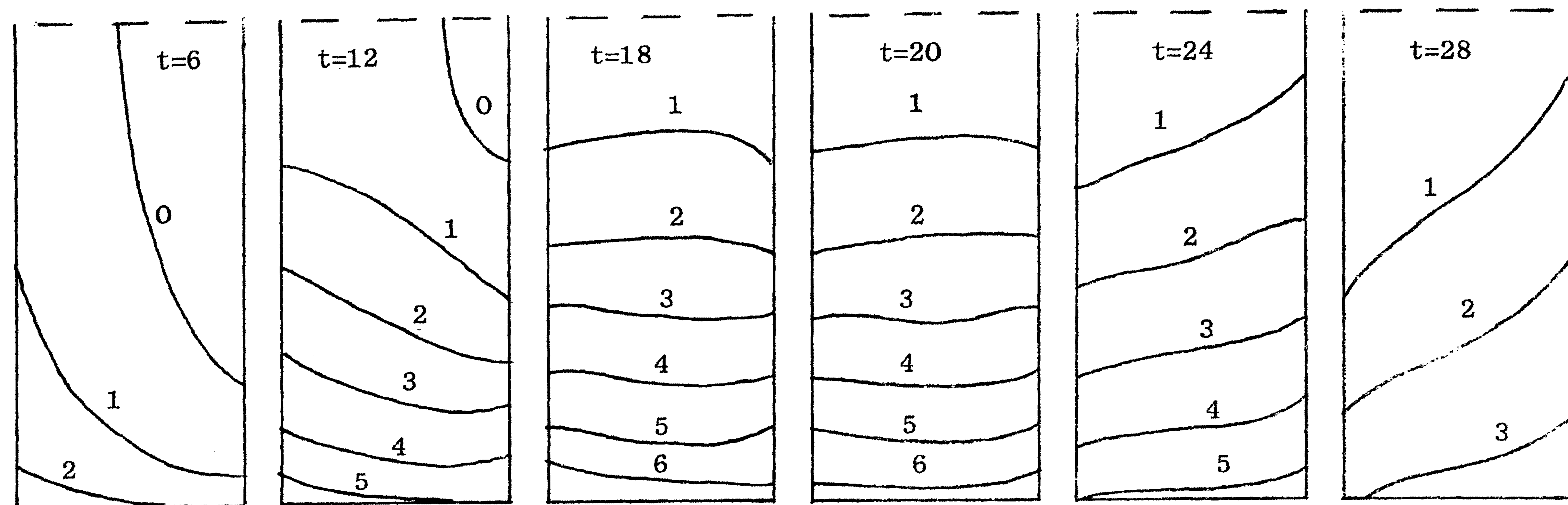
fig.4. Exponential depth. Isohypes due to windfield U=0 , V=-\sin 0.1t
