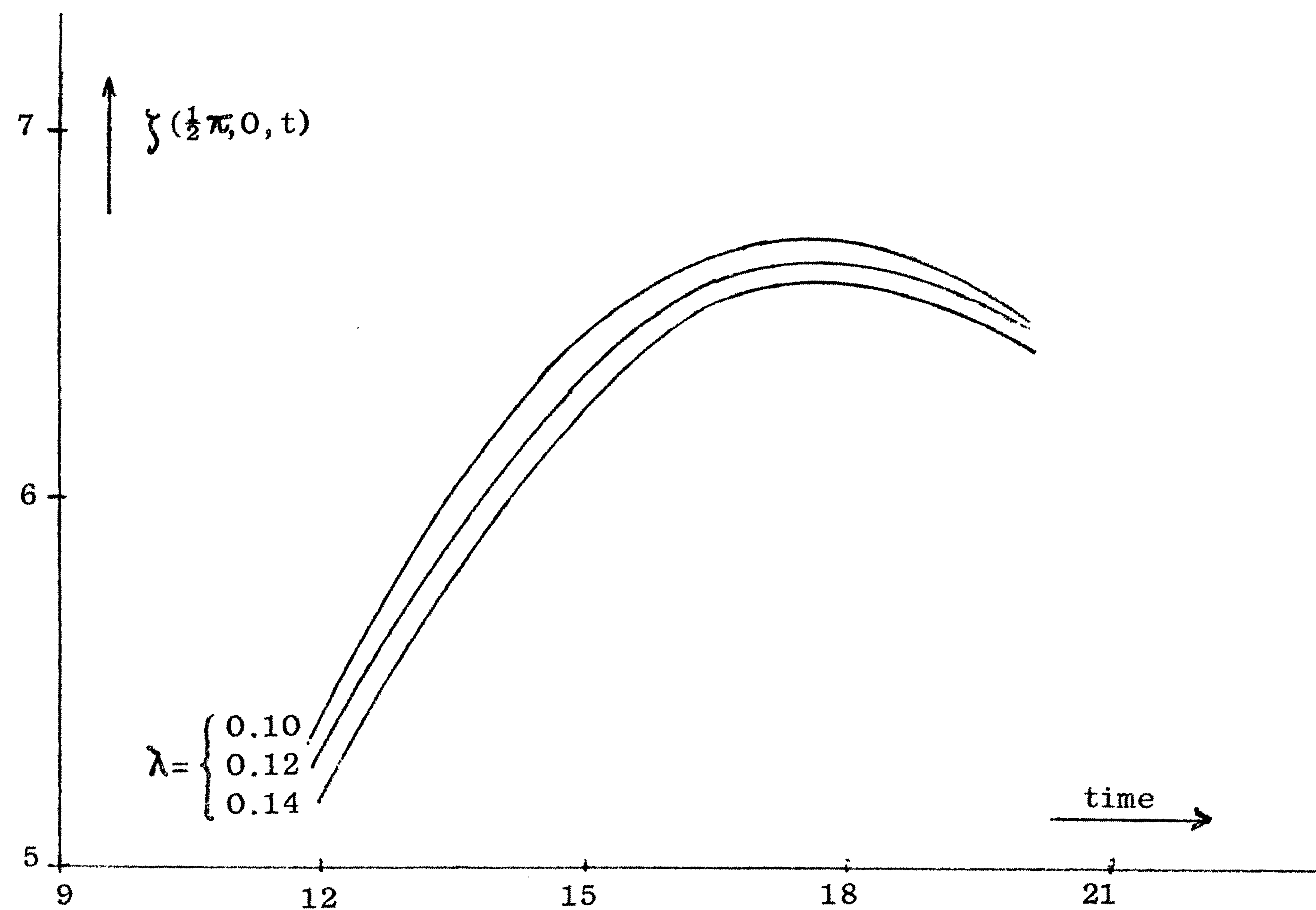
fig.5. Elevation at (\frac{1}{2}\pi, 0) Exponential depth Windfield U = 0 V = -\sin 0.1t \Omega = 0.6 , various values of \lambda .
