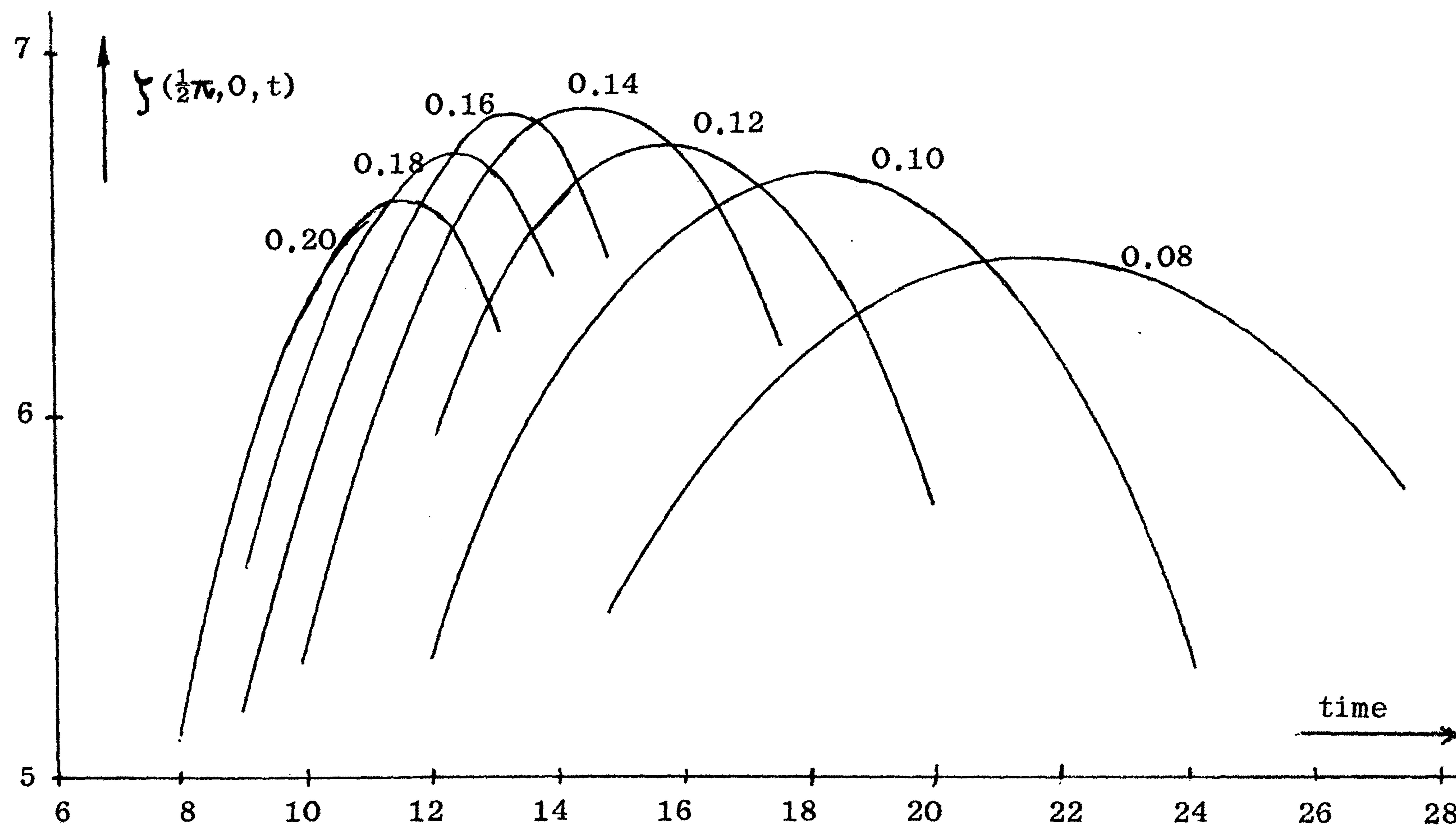
fig.6. Influence of \omega on the elevation at (\frac{1}{2}\pi, 0)
