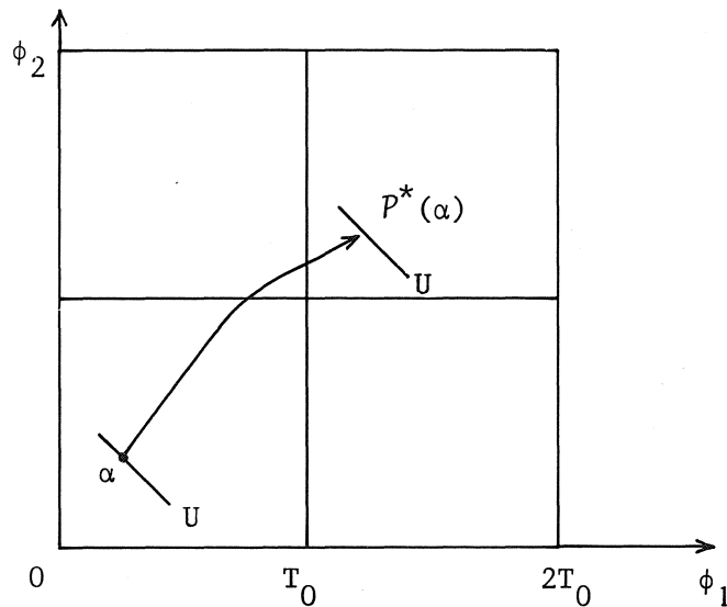
Fig. 3.1. The map \mathcal{P}^* for two oscillators, produced by the trajectories of (3.7.b). The Poincaré map is given by \mathcal{P} = \Phi \mathcal{P}^* \Phi^{-1} . For clarity of the drawing the torus \mathcal{T}^2 = (\mathbb{R}/T_0)^2 has been unrolled.
