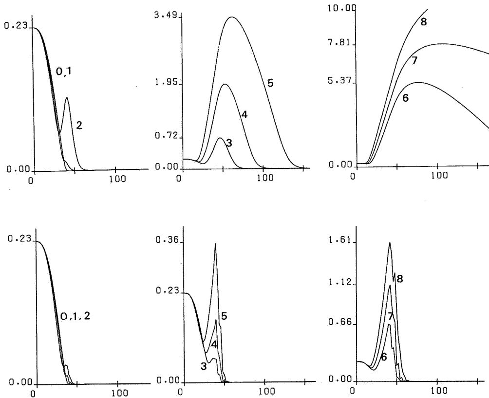
FIGURE 2. The plots represent \log_{10}(1 + \|U^{2n}\|_2) as a function of n . The three upper plots belong to the central scheme, and the three lower ones to the one-sided scheme. The integer numbers i=0(1)8 correspond to \tau according to \tau=1/(40-2i) . Further, h=1/40 , q=1 , \epsilon=0.01 , u(x, 0)=\sin(\pi x) . The case i=0 corresponds to the CFL condition and i=8 yields the maximal \tau -value allowed by condition (3.10a).
