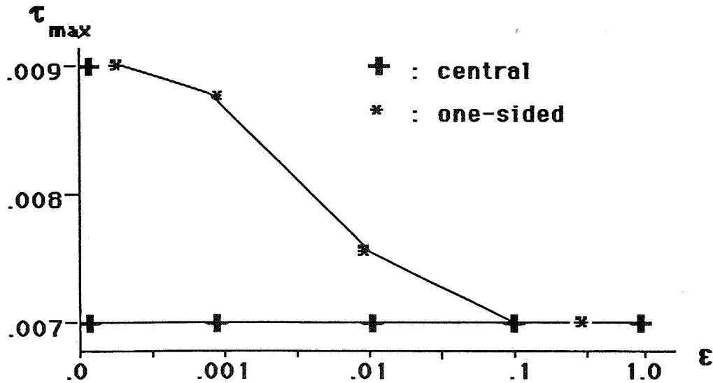
FIGURE 1. Illustration of maximal stepsizes.
