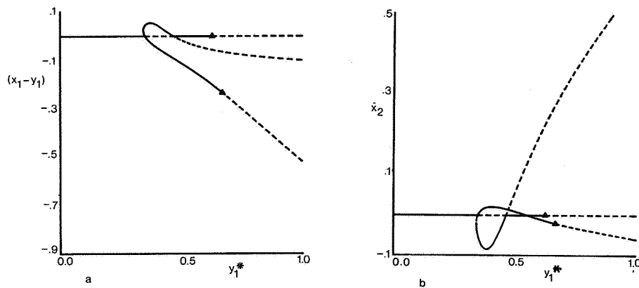
FIGURE 15. As figure 13, but for the wave-number 6 situation.
