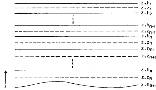
FIGURE 2. Level model for a continuously stratified fluid. Eq. (2.9a) is considered on the levels z = z_n and eq. (2.9b) on z = h_n ( n = 1, 2, \dots, N ).
