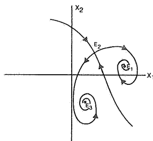
FIGURE 6. Sketch of the phase flow projected onto the x_1-x_2 plane. Initial conditions are chosen in a plane x_3 = \text{constant} .
