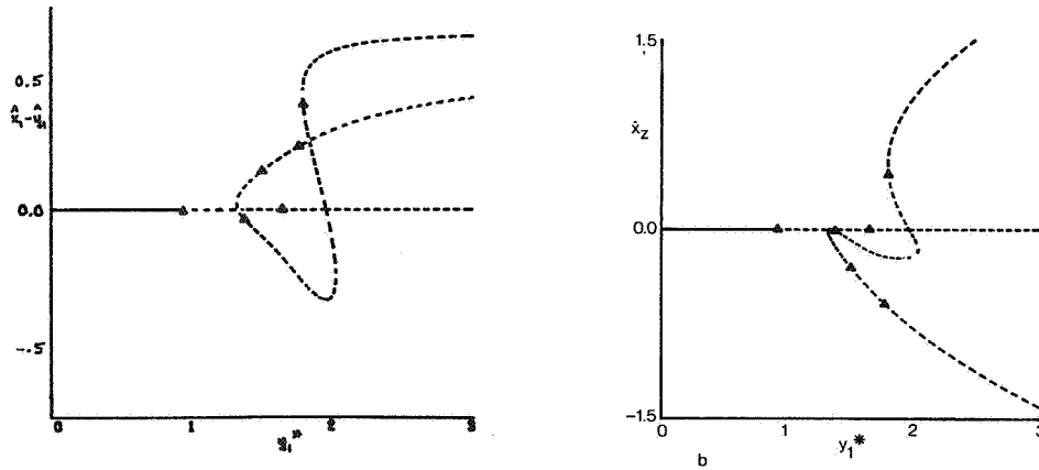
FIGURE 16. As figure 13, but for the twelve component baroclinic model.
