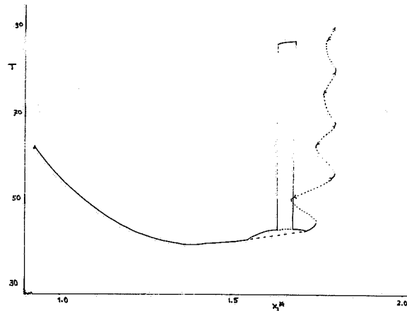
FIGURE 8. Period T of the periodic orbits emanating from the E_3 branch of stationary points as a function of x_1^* , x_4^*=0 , \gamma=1 . Solid curves denote that the orbit is stable, while dashed curves refer to unstable orbits. The symbols -< and -> denote sequences of period doublings and period halvings in a very small region of x_1^* values, respectively.
