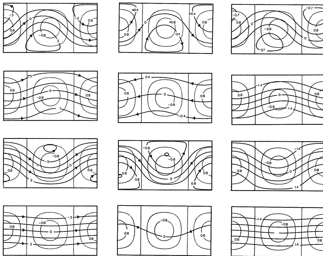
FIGURE 14. Contour plots (solid curves) of the nondimensional streamfunction patterns at the upper level (left) and lower level (middle), as well as the nondimensional potential temperature distribution (right) of the branch 2 (a), branch 3 (b), branch 4 (c) and branch 5 (d) equilibria discussed in the text. Arrows denote the direction of the flow \Delta\psi=1 corresponds to a zonal transport of 2.7 \cdot 10^7 \text{ m}^2 \text{ s}^{-1} , \Delta\theta=1 corresponds to a potential temperature difference of 0.1 \cdot \theta_s , where \theta_s is defined by (2.5). The dashed curves represent contours of topography (km).
