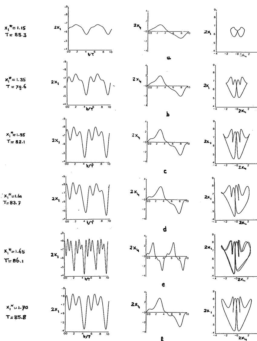
FIGURE 9. Visualization of some stable periodic solutions discussed in section 4.3, see figure 8. Shown are x_1(t/T) , x_4(t/T) and the projection of the orbits onto the x_1 - x_4 plane. Here t is time and T the period.
