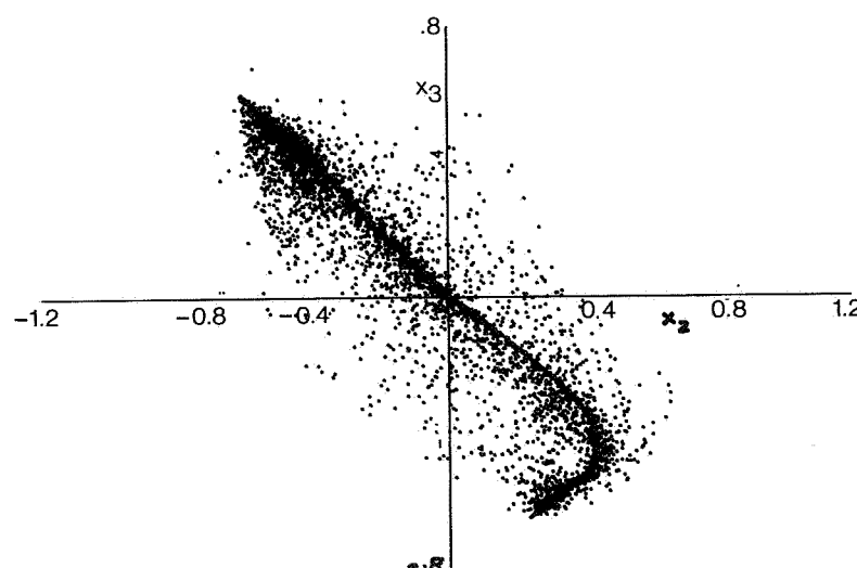
FIGURE 17. Climatology of the (1,1) barotropic wave mode of the twenty component baroclinic model for the demonstration case discussed in the text. Shown are daily values of the x_2 and x_3 component for an integration period of 15 years. Here # denote single mode stationary points of the model, see text.
