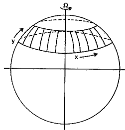
FIGURE 3. The midlatitude channel. The x -coordinate is along lines of constant latitude, the y -coordinate along lines of constant longitude.
