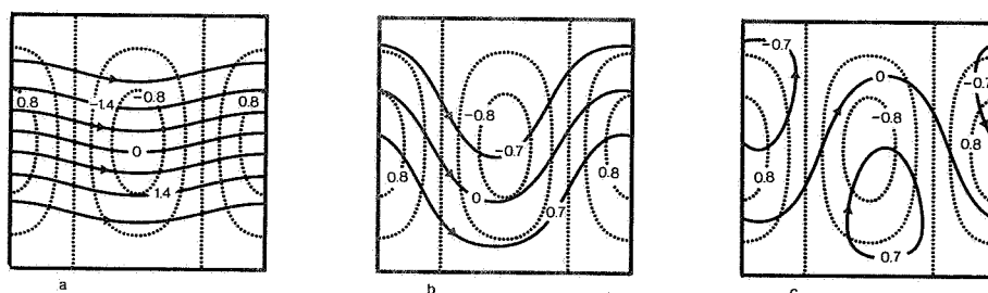
FIGURE 5. Nondimensional streamfunction patterns of the equilibria E_1(a) , E_2(b) and E_3(c) for \gamma=1, x_1^*=2 . \Delta\psi=1 corresponds to a zonal transport of 2.6 \cdot 10^7 \text{ m}^2 \text{ s}^{-1} . The dashed lines represent contours of the topography.
