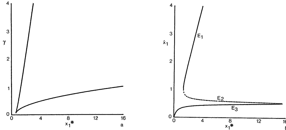
FIGURE 4. a. Bifurcation set in the \gamma, x_1^* -parameter space of the three component model.
