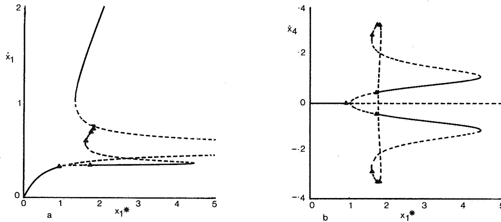
FIGURE 7. As figure 4b, but solution components \hat{x}_1 and \hat{x}_4 of the six component model as a function of x_1^* for x_4^*=0 , \gamma=1 . The triangles denote Hopf bifurcation points.
