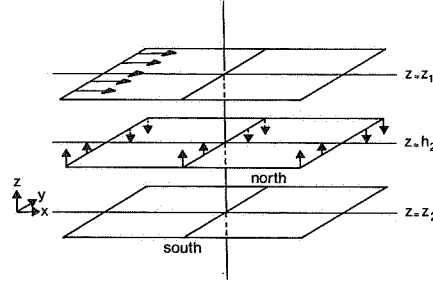
FIGURE 12. Threedimensional circulation pattern of the Hadley equilibrium state defined by (5.4).
