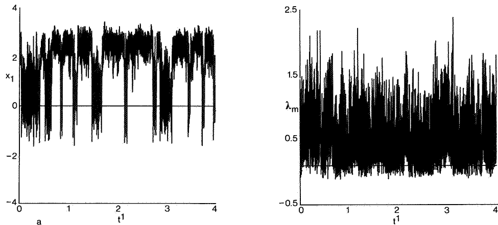
FIGURE 11. a. Nontransient time series of the x_1 component of the ten component model (4.1), which is proportional to the zonal index. The period shown is approximately eight years, for parameter values see text. b. Time series of the maximum real part \lambda_m of the eigenvalues of the phase flow, linearized at each point of the orbit shown in figure 11a.
