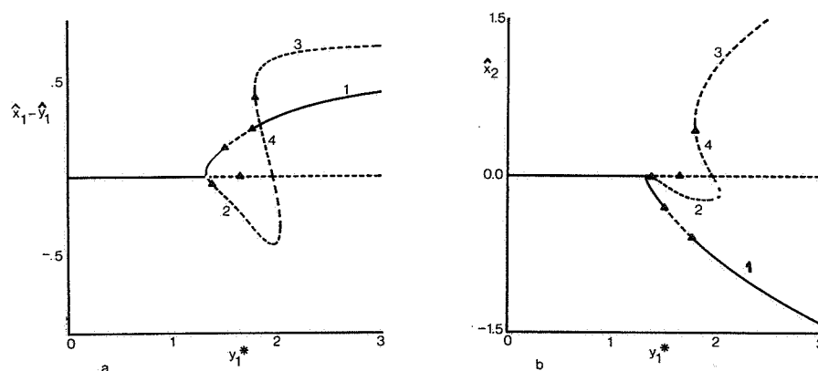
FIGURE 13. Stationary solutions of the six component baroclinic model for the wave-number 3 situation discussed in the text. Shown are (\hat{x}_1 - \hat{y}_1) and \hat{x}_2 as a function of the thermal forcing y_1^* . Branch numbers are also indicated.
