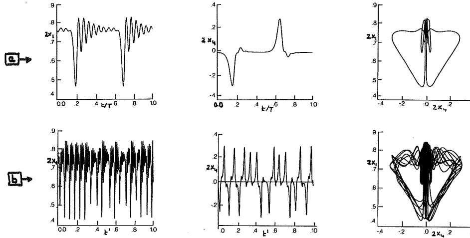
FIGURE 10. a. Numerical approximation of the homoclinic orbit at x_1^* = x_{1,c}^* as a periodic orbit with a large period, here T \approx 120 . Shown are the x_1 and x_4 component as a function of t/T , as well as the projection of the orbit onto the x_1-x_4 plane. b. Chaotic time series for x_1^* = 1.75 started in the unstable equilibrium E_3 . Shown are the x_1 and x_4 component as a function of t' = t/500 - 1 as well as a projection of the trajectory onto the x_1-x_4 plane. Transient effects have already died out before entering the time interval shown.
