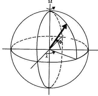
FIGURE 1. Spherical coordinates for the earth.
