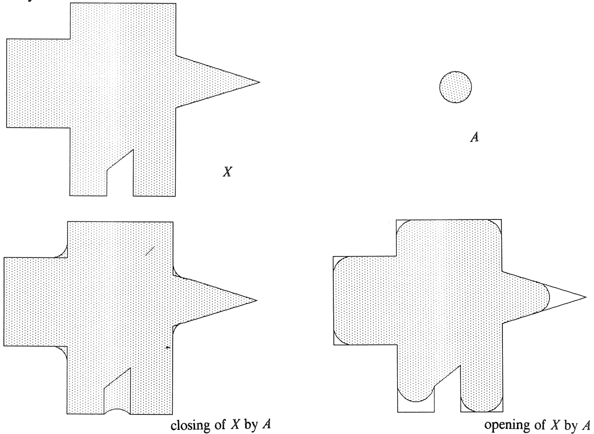
FIGURE 3. Closing and opening in the continuous case
