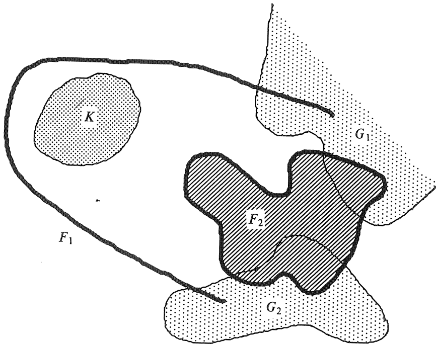
FIGURE 5. F_1 and F_2 both belong to the base element \mathcal{G}^K \cap \mathcal{G}_{G_1} \cap \mathcal{G}_{G_2} .
