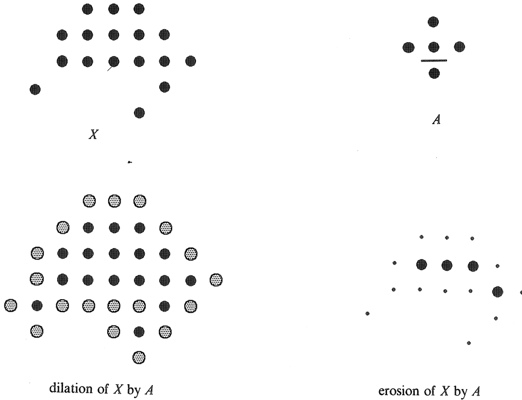
FIGURE 2. Dilation and erosion in the discrete case ● points which belong to X ⊙ points which belong to X \oplus A but not to X ◦ points which belong to X but not to X \ominus A The underlining in A denotes the location of the origin.
