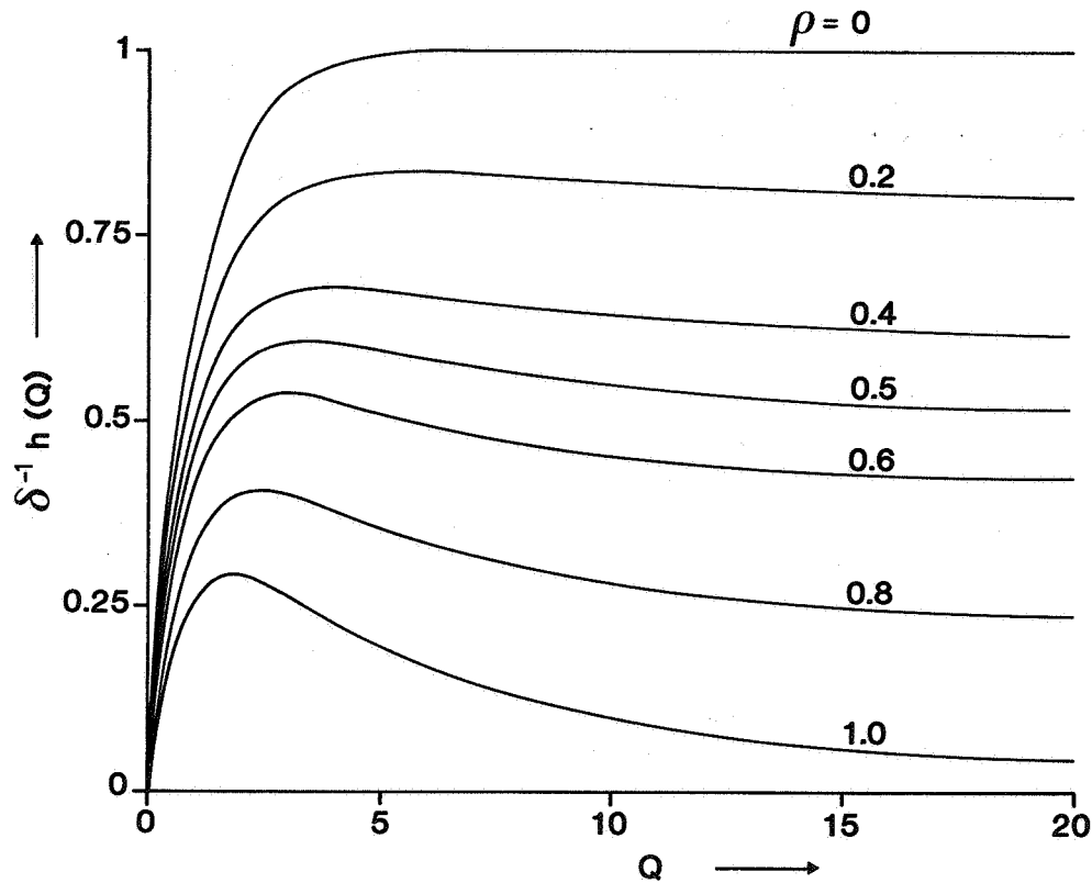
FIGURE 5 The relation between h and Q for \omega=1 , \delta=1 and various values of \rho
