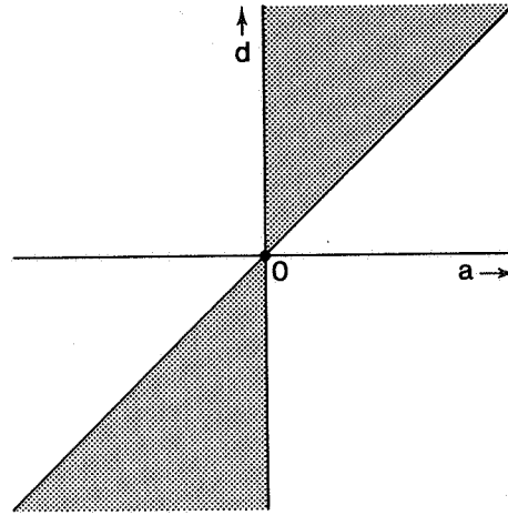
FIGURE 4 The stability region is shaded.
