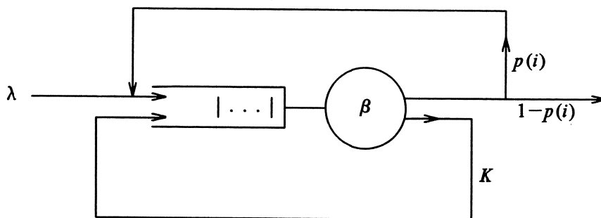
Fig. 5.1 The M/M/1 feedback queue with K additional permanent customers.
