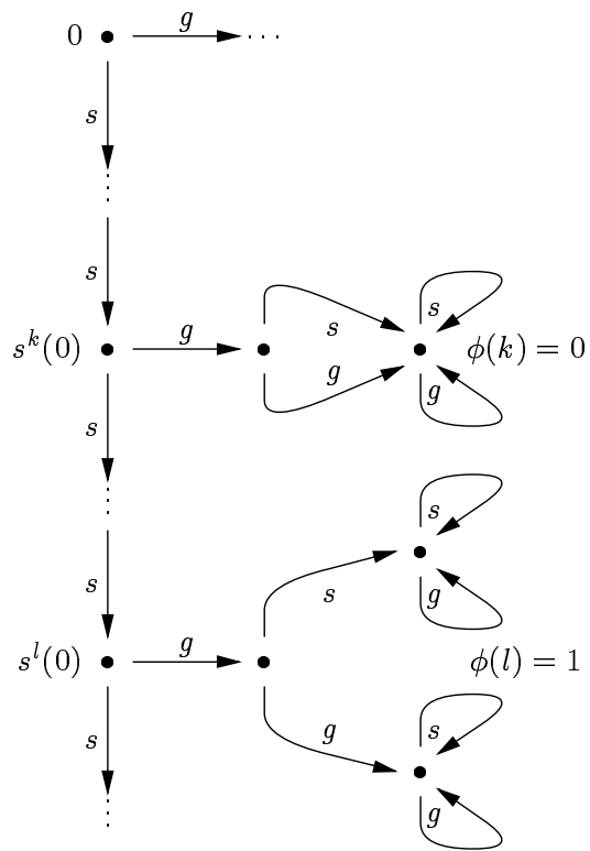
Figure 1: The algebra A_\phi
