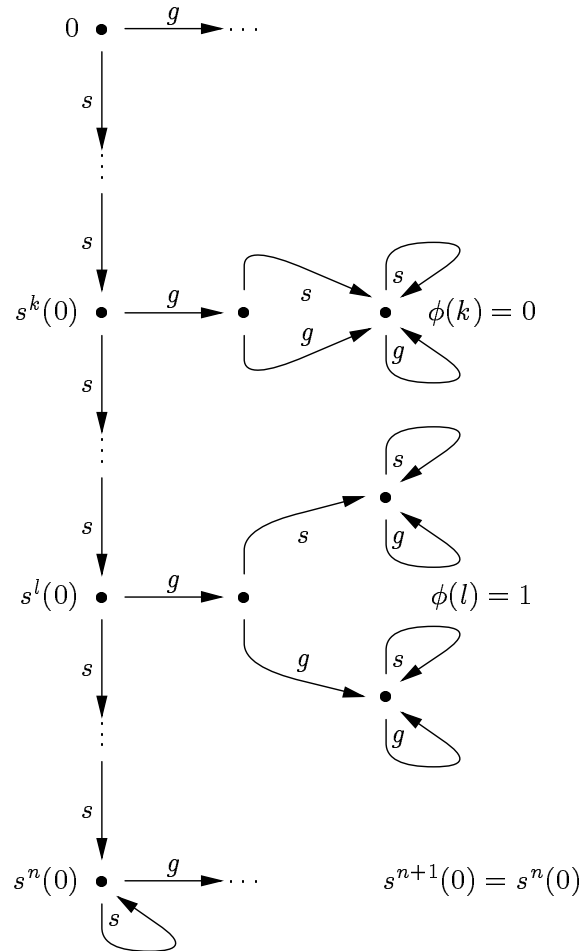
Figure 2: The finite homomorphic image A_{\phi,n}
