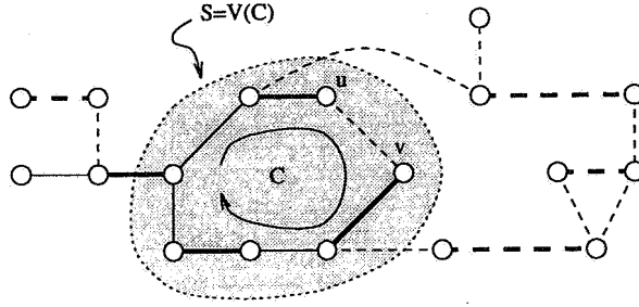
Figure 3: Solid edges are in the alternating forest; bold edges, dashed or not, are in the matching. The shaded region indicates a blossom.
