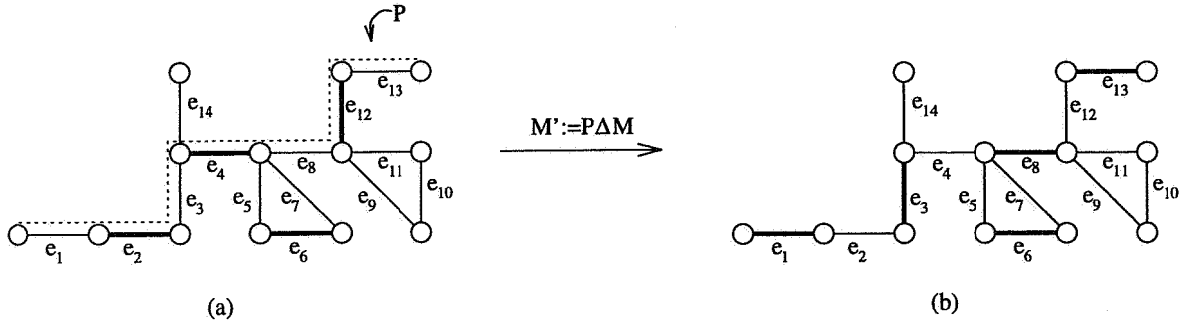
Figure 1: The bold edges are in the matchings M respectively M'
