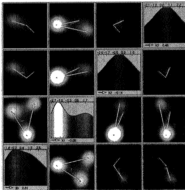
Figure 3: HyperSlice applied to four-dimensional potential function
