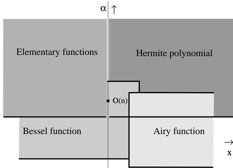
Figure 7.2. When \alpha and n of L_n^\alpha(x) are both large and positive, 4 types of uniform asymptotic expansions and 4 domains are needed to cover the (x, \alpha) -half plane
