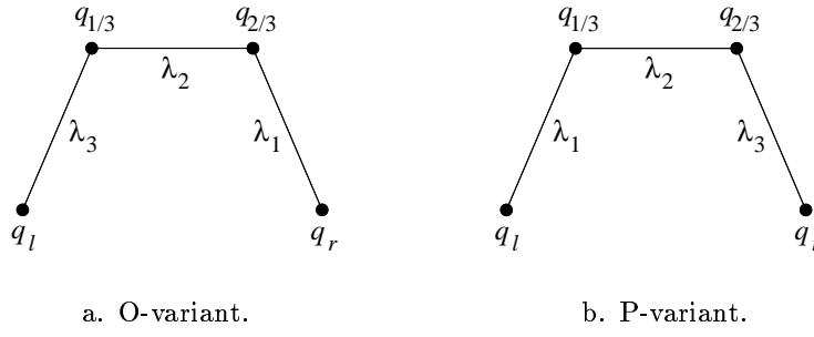
Figure 6: Two variants of Osher-path in state space.
