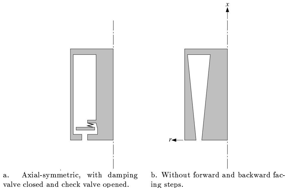
Figure 2: Schematized rebound volumes.
