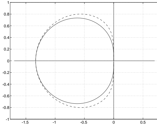
Figure 1: The explicit stability region \mathcal{S} (dashed) and the region \mathcal{D} for the IMEX-BDF2 method.
