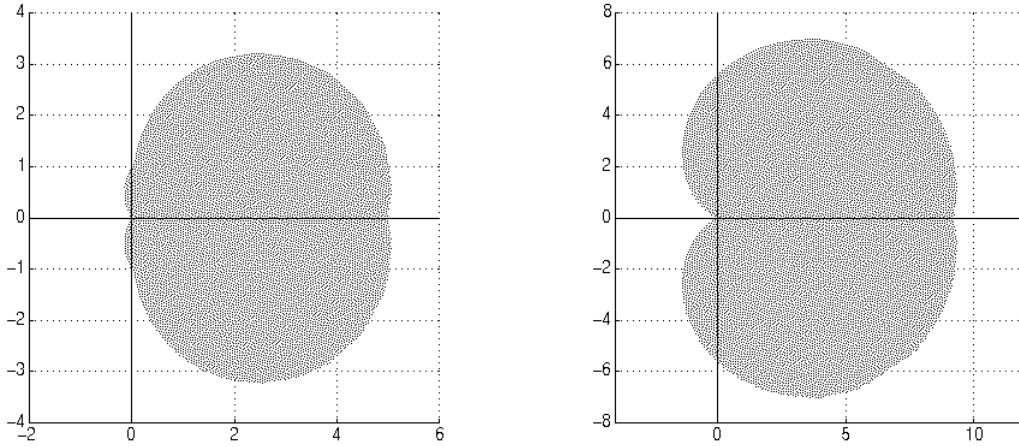
Figure 4: Exterior of shaded region: stability for \mu with arbitrary \lambda \in \mathcal{S} for the IMEX-Adams method with c = 1/2 (left) and c = 1/8 (right).
