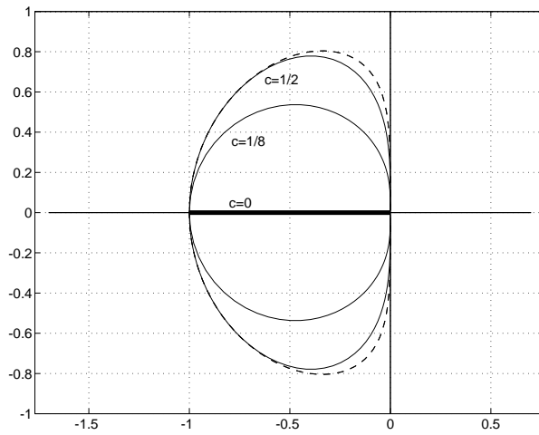
Figure 2: The explicit stability region \mathcal{S} (dashed) and the regions \mathcal{D} for the IMEX-Adams2 methods with c = 1/2, 1/8 and 0 .
