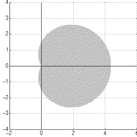
Figure 3: Exterior of shaded region: stability for \mu with arbitrary \lambda \in \mathcal{S} for the IMEX-BDF2 method.
