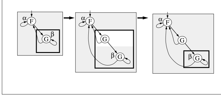
Figure 26. Analysis of \mu -step.
