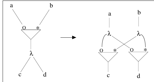
Figure 35. Fan-in and \lambda interaction.
