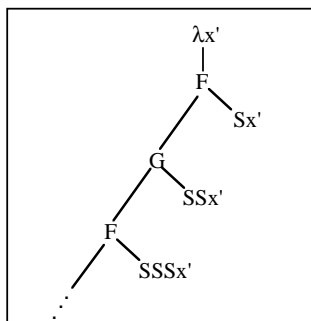
Figure 40. Partial tree.
