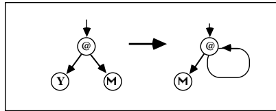
Figure 1. Cyclic Y-rule.
