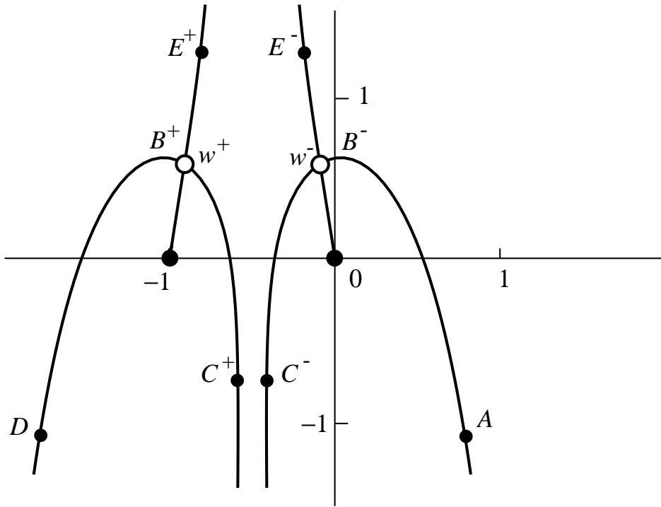
Figure 2.2. The saddle point contours of (2.1) through the saddles at w^\pm for the case z = 1.75 . Saddle point contours are: AB^-C^- for P_n , C^+B^+D for Q_n , AB^-C^- \cup C^+B^+D for E_{n,n} .
