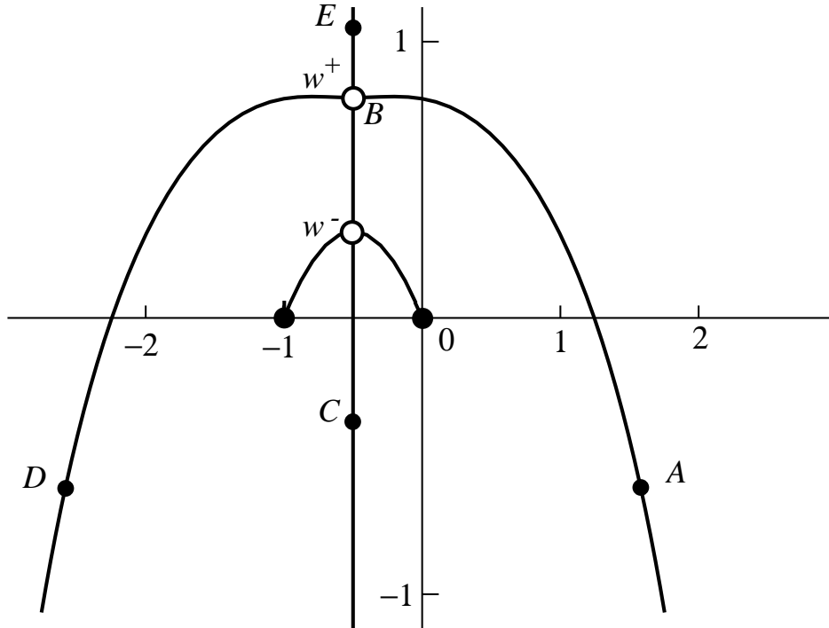
Figure 2.1. The saddle point contours of the integral in (2.1) through the saddles at w^\pm for the case z = 0.9 : ABC for P_n , CBD for Q_n , and ABD for E_{n,n} .
