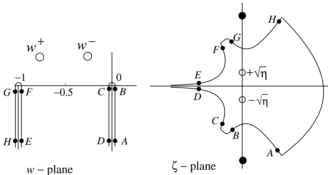
Figure 5.1. Geometrical details of the mapping (3.4) with corresponding points in both planes. The black dots on the imaginary axis are singularities at \zeta = \pm 4.846 \dots i .
