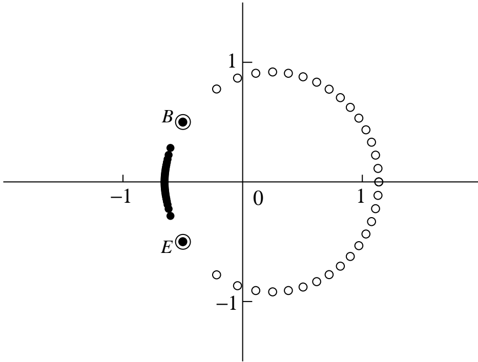
Figure 6.1. Trajectories of the saddle points w^+ (open dots) and w^- (black dots) when z runs through the zeros of P_n , with n = m = 31 . At B and E the saddle points coincide when z = \pm i .
