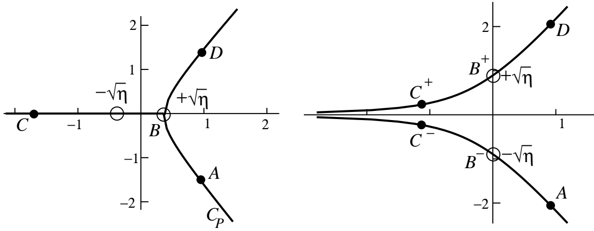
Figure 2.3. The contours in the \zeta -plane and points A, B, C, D that correspond to the points on the contours on the w -plane of Figures 2.1 (with z = 0.9 ) and 3.2 (with z = 1.75 ), with saddle points (open circles) at \pm\sqrt{\eta} .
