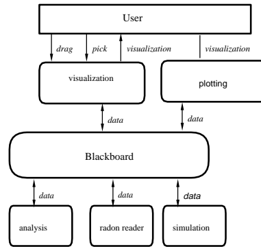
Figure 9: Blackboard configuration of Radon application.
