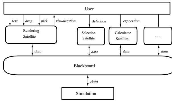
Figure 1: The user view of the blackboard architecture.
