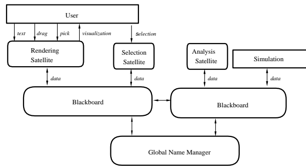
Figure 4: Distributed blackboard architecture.
