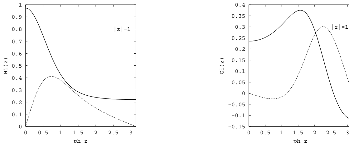
Figure 4.2 The real (solid) and imaginary (dashed) parts of H_i(z) (left) and G_i(z) (right) for |z| = 1 and 0 \leq \text{ph } z \leq \pi .
