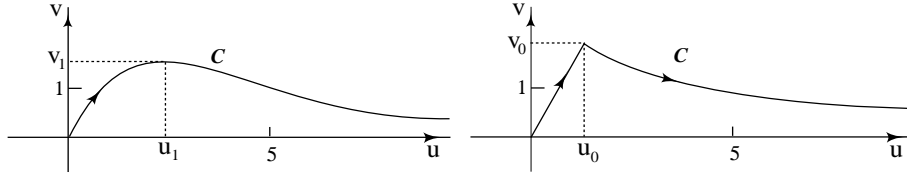
Figure 3.1. The contour \mathcal{C} is defined by (3.4). The left figure is for z inside the sector 2\pi/3 \leq \text{ph } z \leq \pi , and the curve is defined by (3.4). If \text{ph } z = 2\pi/3 the curve in the right figure is defined by (3.8).
