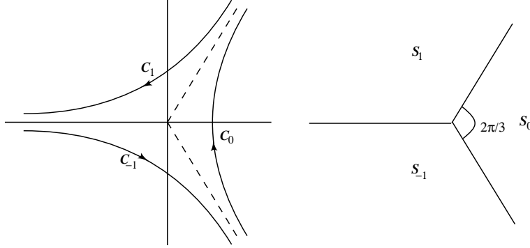
Figure 2.1. Three contours \mathcal{C}_j of integration for the Airy integrals in (2.2), and sectors S_j where \text{Ai}_j(z) are recessive.
