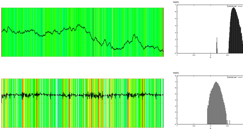
Figure 3: Left: Example time series with local Hurst exponent indicated in colour: fBm with H = 0.6 and the record of healthy heart interbeat intervals. The background colour indicates the Hölder exponent locally, centred at the Hurst exponent at green, colour goes towards blue for higher \hat{h} and towards red for lower \hat{h} . Right: The corresponding log-histograms of the local Hölder exponent.
