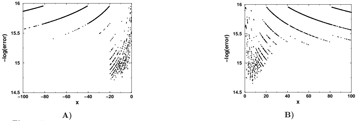
Figure 5. -\log_{10}(\text{error}) for the comparison of the numerical values obtained by our code for Hi(z) (A) (interval [-100 : 0] ) and Gi(z) (B) (interval [0 : 100] ) with MacLeod's code.
