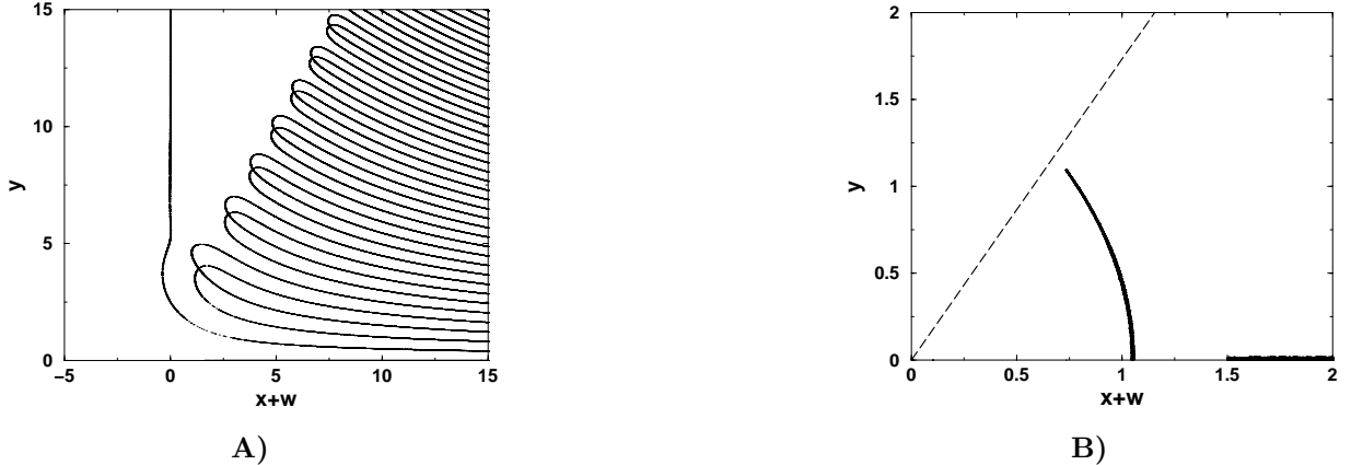
Figure 2. Points where the relative deviations for the computation of the phase of \text{Hi}(z+w) (A) through (4.1) and \widetilde{\text{Hi}}(z+w) (B) through (4.3) are greater than 10^{-12} compared with direct computation. In Figure B we also plot the line \text{ph}(z+w) = \pi/3 , which is the limit of validity of the scaling for \text{Hi}(z+w) .
