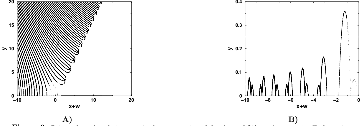
Figure 3. Points where the relative error in the computation of the phase of \text{Gi}(z+w) , comparing Taylor series around w = 0 with the direct computation by the code GIZ, is greater than 10^{-12} (A). Similarly, the corresponding discrepancies found in the evaluation of the phase of \widetilde{\text{Gi}}(z+w) within a relative accuracy of 10^{-12} are shown (B).
