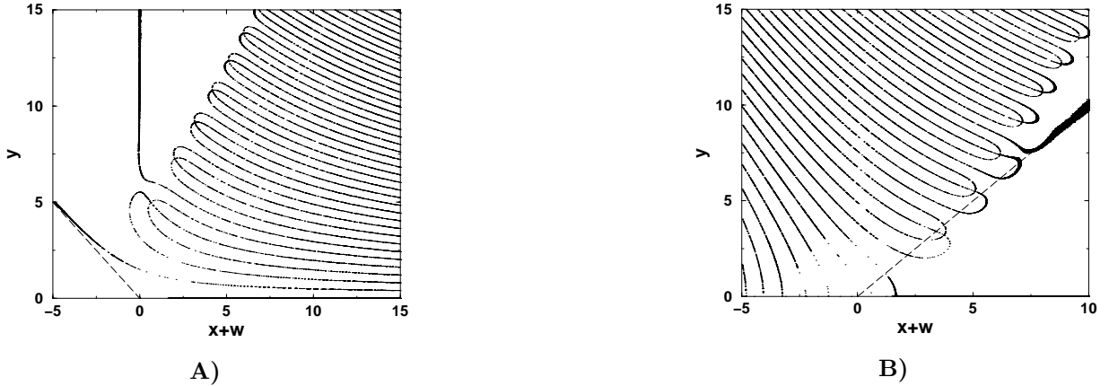
Figure 4. Points where the relative deviations in the computation of the phase of \text{Hi}'(z+w) (A) and \text{Gi}'(z+w) (B) are greater than 10^{-12} (comparing Taylor series around w = 0 with direct computation). The rays \text{ph}(z+w) = 3\pi/4 (A) and \text{ph}(z+w) = \pi/4 (B) are also shown (dashed lines).
