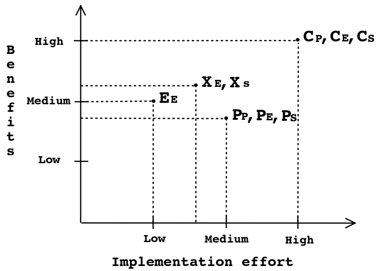
Figure 2: Implementation cost-benefit trade-off for feasible pairs of design and implementation pattern. Pairs are denoted I_J where I is an implementation pattern (interpreter/compiler (C), preprocessor (P), embedding (E), and extensible compiler/interpreter (X)), and J is a design subpattern (piggyback (P), specialization (S), and extension (E)).
