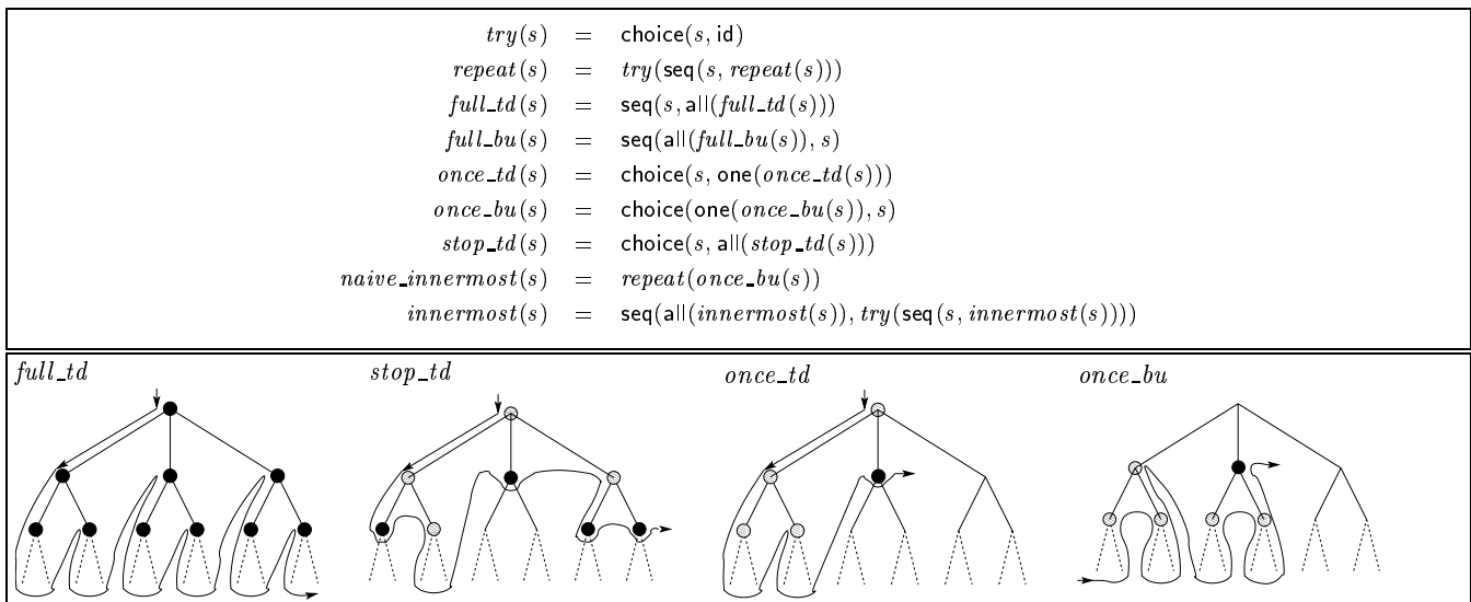
Figure 6: Some defined strategy combinators
