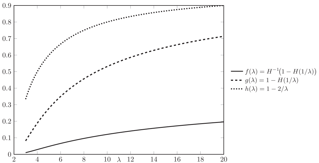
FIGURE 1 Graphs of f, g, h (from bottom to top) over the domain [3, 20] .
