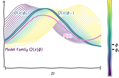
Figure IV.2.: Schematic representation of the fmPE (Def. IV.13): among a family of models Q(x|\phi) [Eq. (IV.52), colored as per the colorbar based on the value of the parameter \phi ] supported on \mathcal{D} , the one that minimizes the inverse KL divergence with P(x) (Def. IV.7) is Q(x|\phi^*) . The target distribution P(x) is the final result of the filtered-QPE scheme represented in Fig. IV.1. We also highlight the model distribution for the ideal value of \phi = \phi_0 : Q(x|\phi_0) – the difference between \phi_0 and the optimal parameter \phi^* is the bias of the fmPE.
