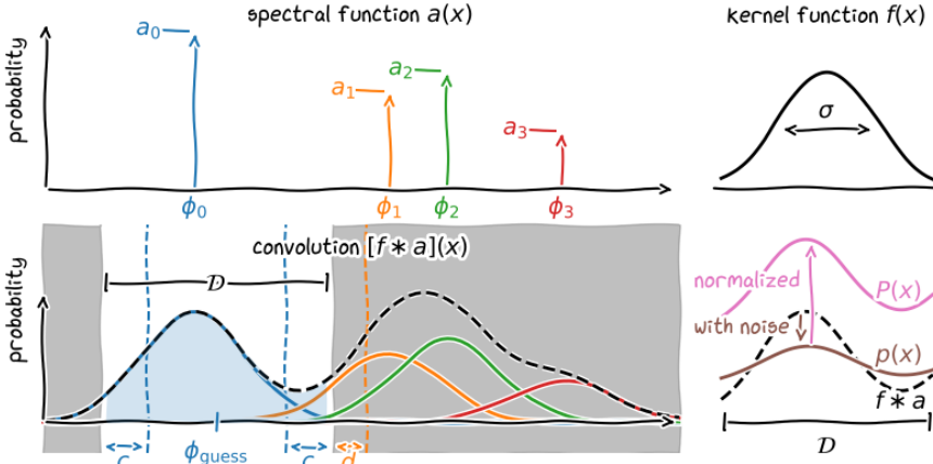
Figure IV.1.: Schematic plot illustrating the construction of the signal distribution of a filtered QPE experiment. (Top left) A unitary operator U and initial state |\psi\rangle define the spectral distribution a(x) in Def. IV.2 – a sum of Dirac deltas centered at the eigenphases \phi_j of U with amplitudes a_j . (Top right) We define a kernel function f(x) (Def. IV.3), with a shape and width \sigma depending on the details of the circuit. (Bottom left) The QPE circuits can sample from a distribution obtaining by convolution of a and f – the distribution in Def. IV.3, shown by the dashed black line. (The colored lines indicate the contributions of each eigenphase \phi_j to the total distribution.) The filtering procedure discards all samples outside of a filtering region \mathcal{D} , which is chosen assuming that the phase of interest \phi_0 is within the interval (farther than an inner buffer distance c from the interval edges) and all other phases are outside the interval (farther than an outer buffer distance d from the interval edges) – see Def. IV.6. The unnormalized distribution of filtered outcomes in the absence of noise is highlighted in blue. (Bottom right) Adding noise to the distribution f * a yields the distribution p(x) (Def. IV.5). Normalizing this distribution within the filtering interval \mathcal{D} we obtain the filtered noisy distribution P(x) (Def. IV.7).
