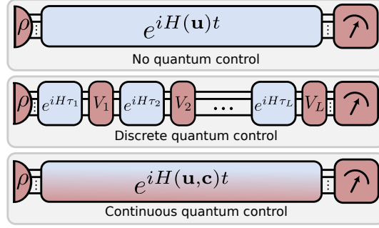
Figure V.1: Schematic quantum circuit diagrams of the three experimental models that we consider in this work. Colors denote when the experimentalist has complete control (red), some control (light blue-red gradient), or no control (light blue) over the operation. We assume the experimentalist has the freedom to specify state preparation (half-ellipse) and measurement (dial symbol). Further, during time evolution (rectangles) we assume the freedom to specify the evolution times t/\tau_i , and the instantaneous quantum operations V_i (in the discrete quantum control model), or the control parameters \mathbf{c} (in the continuous quantum control model). In the discrete control model, we assume the quantum operations V_i are unitary but allow them to act on an arbitrary number of ancilla qubits (not shown), and we hide the dependence of H on the unknown parameters \mathbf{u} for clarity.
