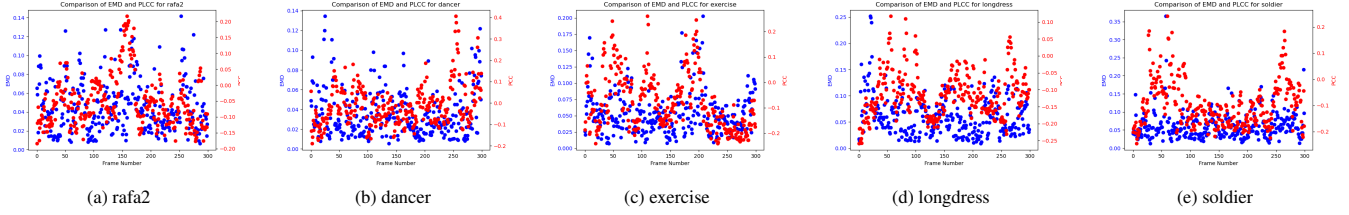
Figure 7: Similarity of point cloud saliency maps between task-free and task-dependent scenarios through EMD (•) and PCC (•) for the shared 5 sequences per frame, separately.
