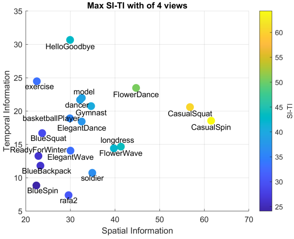
Figure 2: Distribution of SI and TI of 19 source dynamic point clouds from 3 datasets, the color value is computed by \sqrt{(SI^2 + TI^2)} .
