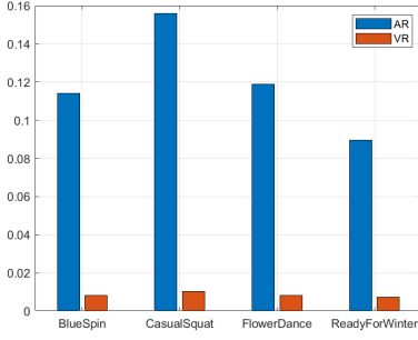
Figure 10: The average ratio of the VoI for the shared 4 dynamic point cloud sequences in AR and VR.
