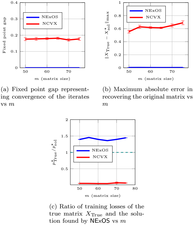
Fig. 4 Affine rank minimization problem: comparison between solutions found by NExOS and NCVX algorithm by [25].
