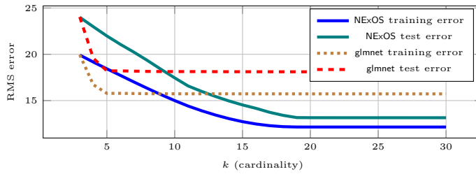
Fig. 3 RMS error vs k (cardinality) for the weather prediction problem.
