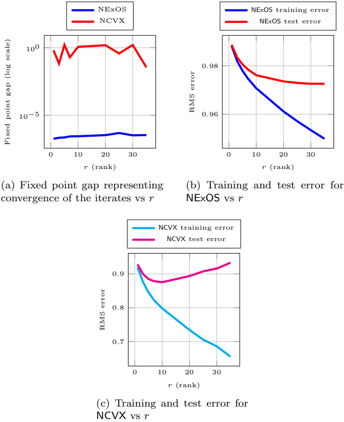
Fig. 5 Matrix completion problem: comparison between solutions found by NExOS and NCVX algorithm by [25].
