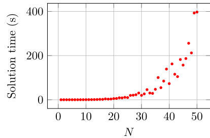
Fig. 1 Numerical results for computing locally optimal stepsizes by solving (25) with the first two stages of the BnB-PEP Algorithm. Global optimality of the stepsizes are verified for N = 1, 2, \dots, 25 . (Left) Worst-case performance of f(x_N) - f_* vs. iteration count N . (Right) Runtimes of the BnB-PEP Algorithm (including Stages 1 and 2 but excluding Stage 3)
