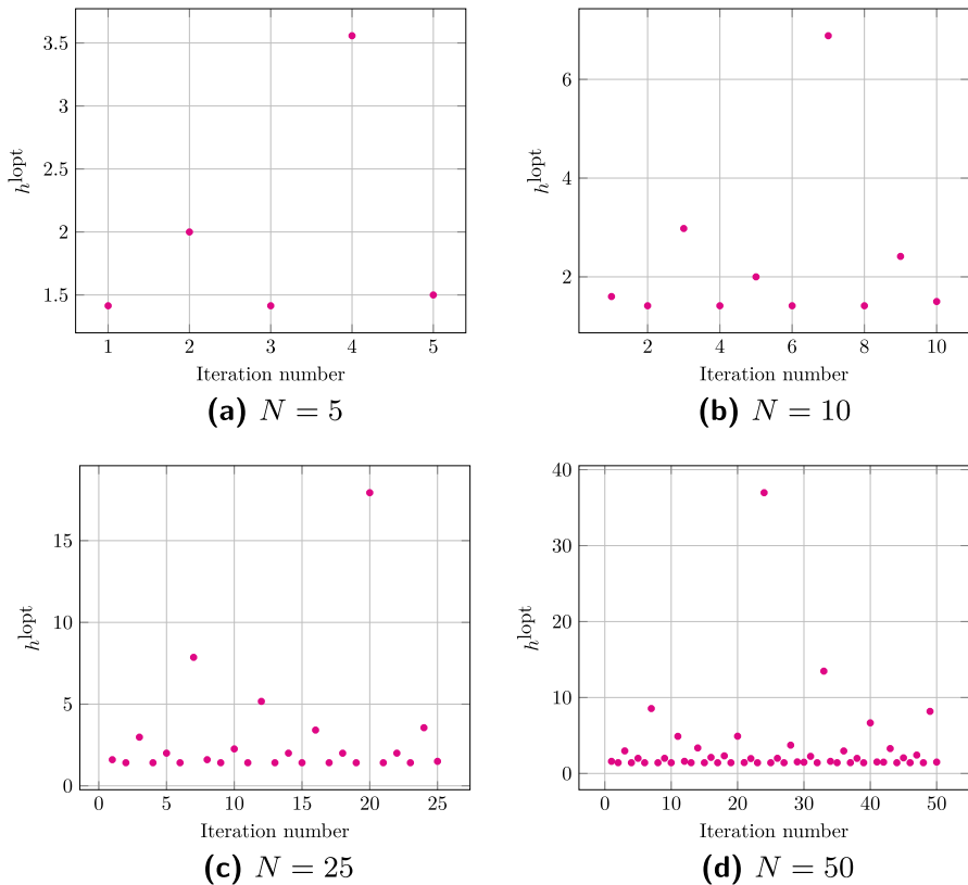
Fig. 3 Locally optimal stepsizes h_i^{\text{lopt}} vs. iteration number for N = 5, 10, 25, 50 with L = 1 . These optimized methods utilize long steps h_i > 2/L for some i , much alike how Young’s method [88] uses long steps satisfying 1 < h_i < L/\mu for some i to achieve an accelerated rate for L -smooth and \mu -strongly convex quadratics
