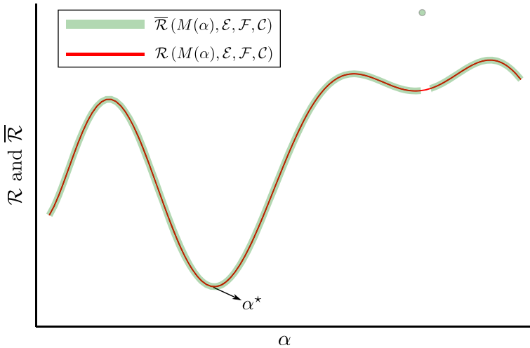
Fig. 7 Illustration of \mathcal{R}(M(\alpha), \mathcal{E}, \mathcal{F}, \mathcal{C}) and \bar{\mathcal{R}}(M(\alpha), \mathcal{E}, \mathcal{F}, \mathcal{C}) when \mathcal{R}(M(\alpha), \mathcal{E}, \mathcal{F}, \mathcal{C}) is continuous. If \alpha^* \in \operatorname{argmin} \bar{\mathcal{R}}(M(\alpha), \mathcal{E}, \mathcal{F}, \mathcal{C}) satisfies \alpha^* \in A^{\text{nice}} , then \alpha^* \in \operatorname{argmin} \mathcal{R}(M(\alpha), \mathcal{E}, \mathcal{F}, \mathcal{C}) , even if there is a duality gap
