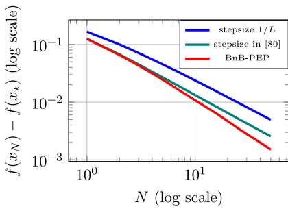
Fig. 1 Numerical results for computing locally optimal stepsizes by solving (25) with the first two stages of the BnB-PEP Algorithm. Global optimality of the stepsizes are verified for N = 1, 2, \dots, 25 . (Left) Worst-case performance of f(x_N) - f_* vs. iteration count N . (Right) Runtimes of the BnB-PEP Algorithm (including Stages 1 and 2 but excluding Stage 3)
