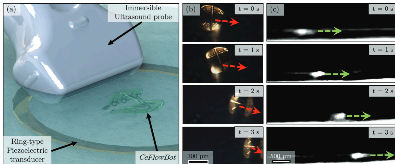
Figure 5. a) Schematic of the experimental setup used for ultrasound (US) imaging of acoustically-actuated CeFlowBot (details in Experimental Section). Time-stamps of the motion of CeFlowBot visualized using b) optical and c) US imaging. The arrows indicate direction of motion of the CeFlowBot (Movie S4, Supporting Information).
