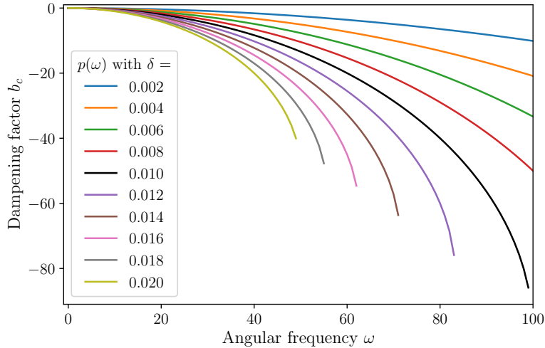
Figure 9. Divergence boundary depending on \delta \in \{0.002, \dots, 0.02\}
