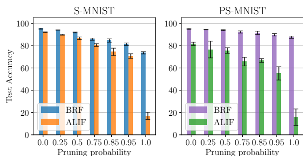
Figure 7. Test accuracy vs pruning probability for (a) S-MNIST and (b) PS-MNIST. 1.0 pruning indicate no recurrent weights.
