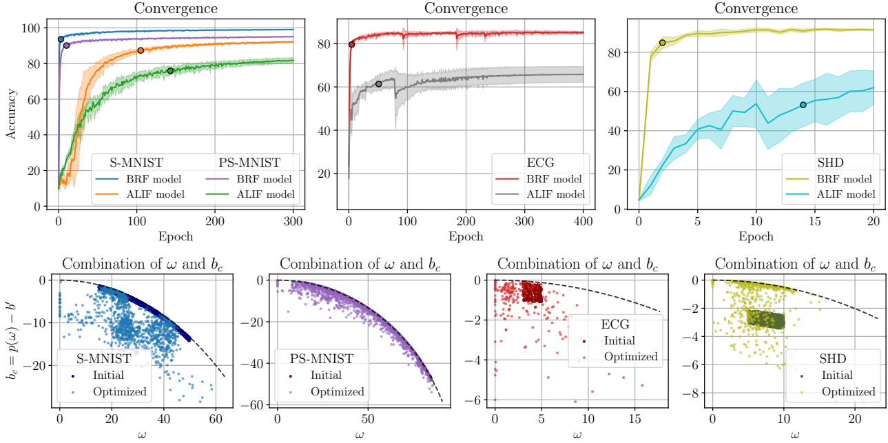
Figure 5. Top row: S-MNIST, PS-MNIST, ECG, and SHD learning curve between BRF and ALIF model. Each curve averaged per epoch (solid line) with standard deviation (shaded area) over five runs. The dot on the accuracy curves depict the point at which 95 % of the final accuracy was reached. Bottom row: S-MNIST, PS-MNIST, ECG, and SHD initial and optimized BRF parameter combinations: angular frequency \omega and b-offset b' for all runs. Dashed line is the divergence boundary.
