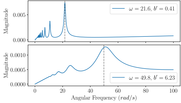
Figure 3. RF neuron frequency response plots for exemplary omega \omega and b-offset b' combinations with \delta = 0.001 .
