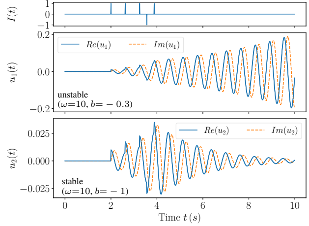
Figure 1. Membrane dynamics of two RF neurons. The four excitatory input spikes are in phase with the neuron’s angular frequency \omega = 10 . The inhibitory spike at half-phase enhances the sensitivity of the neuron to forthcoming excitatory input. Depending on its parameterization, the neuron exhibits divergence behavior (top) with b = -0.3 and \delta = 0.01 or convergence behavior (bottom) with b = -1 . I(t) \in \mathbb{R} and u_1(t), u_2(t) \in \mathbb{C} refer to the injected current and the membrane potential of the neuron, respectively.
