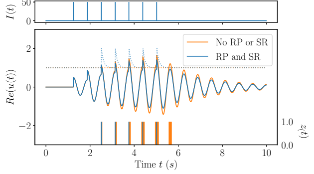
Figure 2. Membrane potential u(t) and spiking response z(t) of an RF neuron without refractory period (RP) or smooth reset (SR) (orange) compared to both (blue) for the given input signal I(t) .
