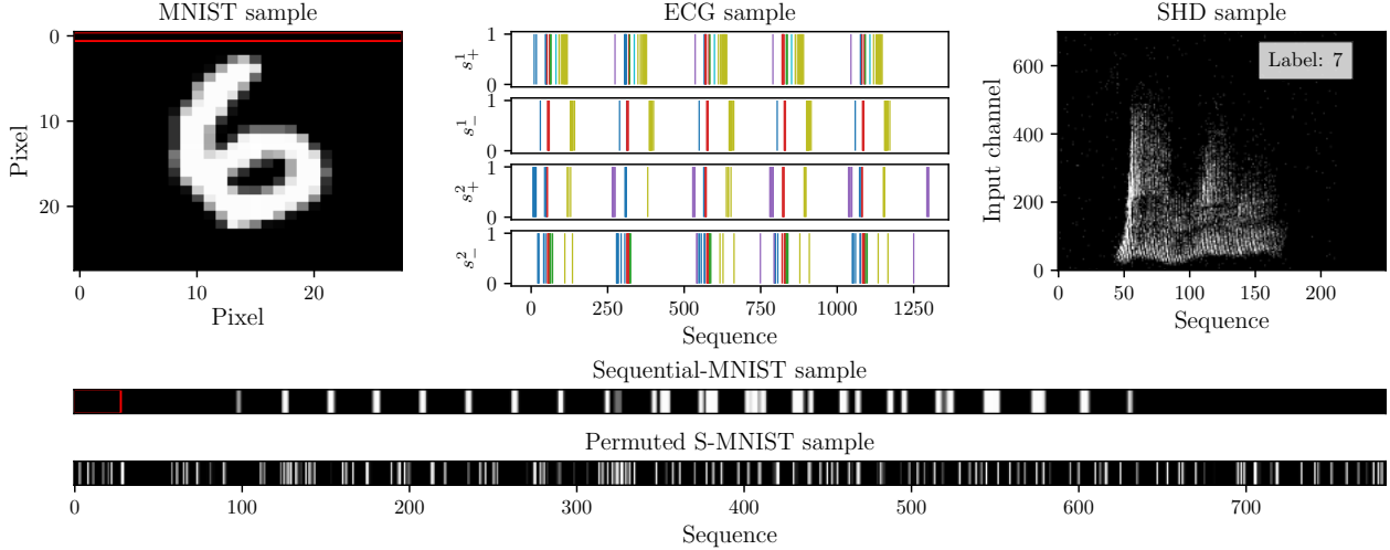
Figure 4. Overview over the datasets. Exemplary MNIST image and its corresponding sequential and permuted representations. Common pixel row outlined in red on MNIST and S-MNIST sample. ECG sample after level cross encoding. SHD sample after preprocessing.
