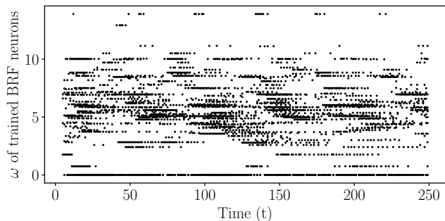
Figure 6. Raster plot of network activity for an SHD sample with label 10 after training. The BRF neurons are sorted by their angular frequency. Black dots denote output spikes.
