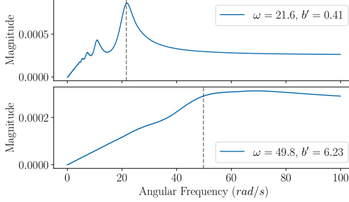
Figure 8. HRF neuron frequency response plots for exemplary omega \omega and b-offset b' combinations with \delta = 0.001 .
