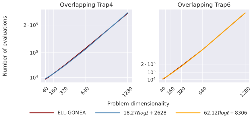
Figure 3.4.4. The curve a \log \ell + b given by the theoretical complexity of \mathcal{O}(\ell \log \ell) fitted to the actual number of evaluations. The values of the empirical results are averaged over 30 runs. The coefficients a and b of the fitted curves are shown in the legend. R^2 coefficients of the fittings are > 0.999 suggesting that the theoretical complexity matches with the empirical one.
