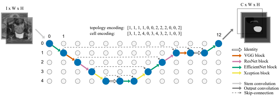
Figure 6.3.2. The scheme of network architectures in the proposed search space and an example U-Net-like architecture. Each circle represents feature maps (a three-dimensional tensor), the blue ones are used in the shown architecture. Feature maps at depth j (from 0 to 4) have 2^j smaller spatial resolution and 2^j more channels than the feature maps after applying stem convolution (in the left upper corner). Each architecture is defined as a sequence of N = 12 cells (represented by arrows). Each cell is defined by two discrete variables: its main block specification (five different options), and its type: normal (horizontal arrows), downsampling (downward arrows), or upsampling (upward arrows). Skip-connections are added using fixed rules (see Section 6.3.3). A stem convolutional block translates an input image to feature maps with 32 channels. An output convolutional block translates corresponding feature maps to segmentation masks.
