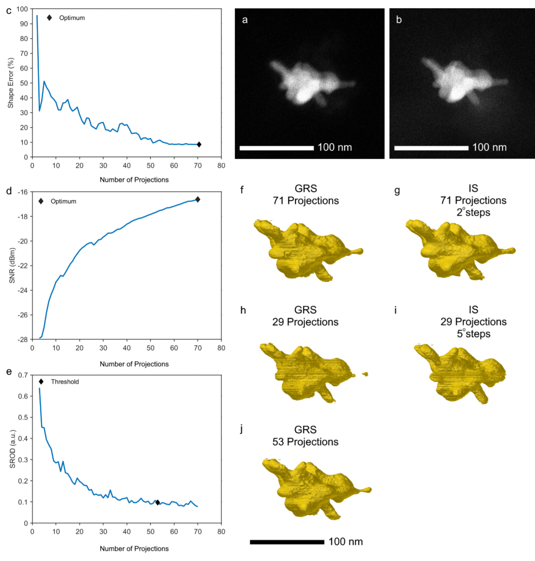
Fig. 8 8^\circ projections of Au/Pd NS before (a) and after (b) collection of three tilt-series (IS 2^\circ , 5^\circ increment and GRS 71 projections). The shape error as a function of the number of projections (c) for GRS reconstructions was determined by comparison to the IS reconstruction with a 2^\circ increment. The SNR (d) and SROD (e) were determined in real-time using TUOTA. The Au/Pd NS was reconstructed with 71 (f-g) and 29 projections (h-i) for GRS and IS. The GRS tilt-series was also reconstructed with the optimum number of projections determined from the SROD threshold (j).
