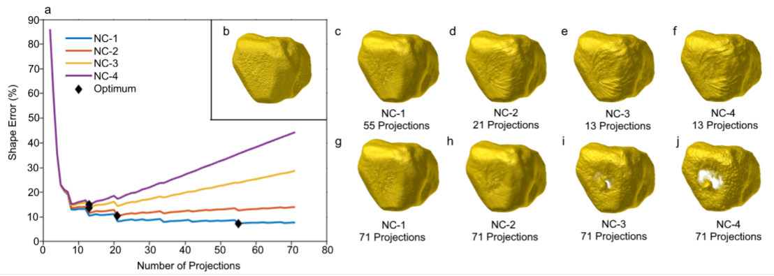
Fig. 6 (a) Shape error as a function of the number of projections for NC1-4 nanocages and their determined optimum number of projections with GRS acquisition scheme. (b) Inset: nanocage before beam damage simulation. 3D reconstruction of NC-1-4 with their optimum number of projections (c-f) and 71 projections (g-j).
