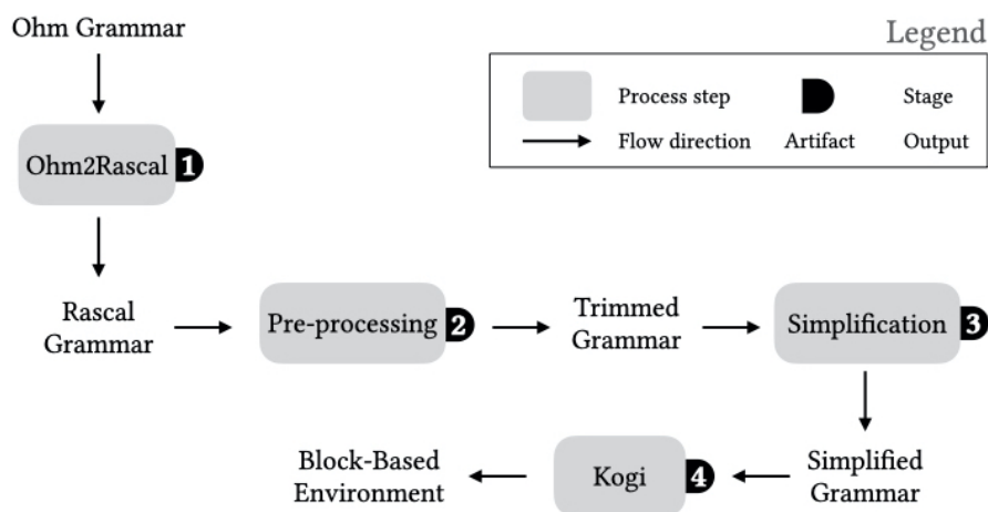
Figure 8.2: S/Kogi's architecture.
