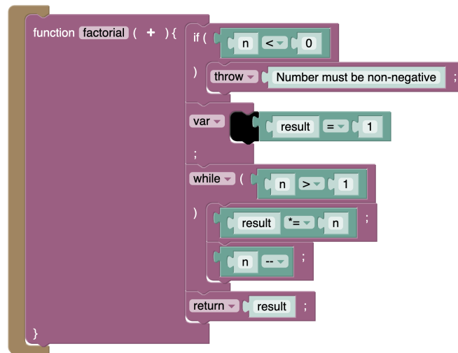
Figure C.6: Example program using the JavaScript environment generated by S/Kogi.
