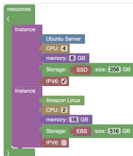
Figure C.7: Example program using the CCL environment generated by Kogi.
