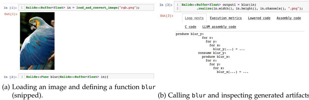
Figure 2.7: Halide notebook.
