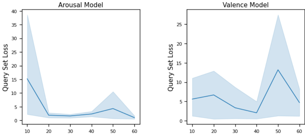
Figure 6.13: RECOLA : Distribution of Query Set Contrastive Loss ( L_q ) for different cases
