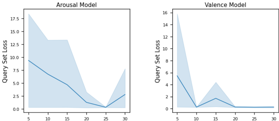
Figure 6.4: K-EmoCon : Distribution of Query set Contrastive Loss ( L_q ) for Baseline Model across Participants
