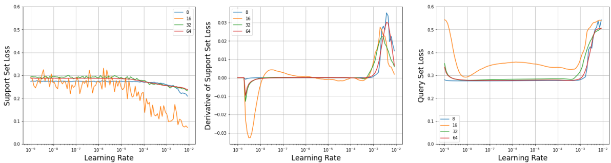
Figure 6.3: K-EmoCon : Learning-rate Range Test for Valence Model
