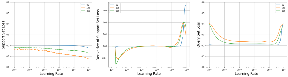
Figure 6.12: RECOLA : Learning rate Range Test Contrastive Loss for Valence Model
