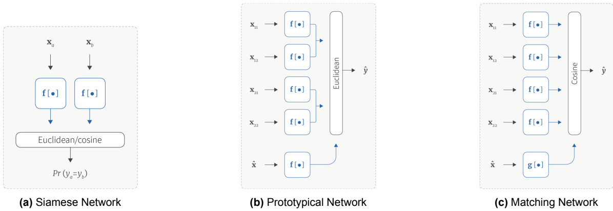
Figure 5.1: Metric Learning Method Architectures (adapted from [111])
