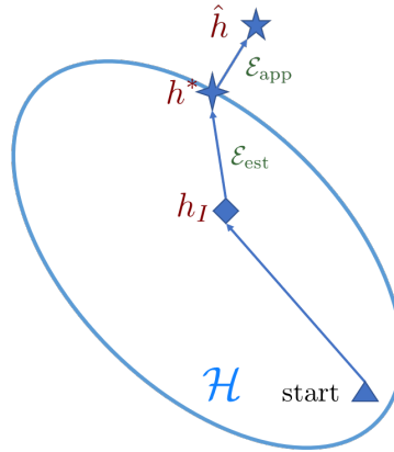
Figure 2.10: Illustration of the Few Shot Learning Problem (adapted from [105])
