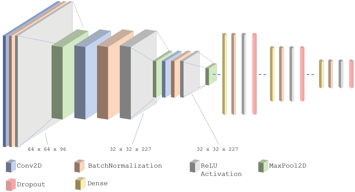
Figure 5.5: Embedding Architecture for Mel Spectrograms [modified from [66]]
