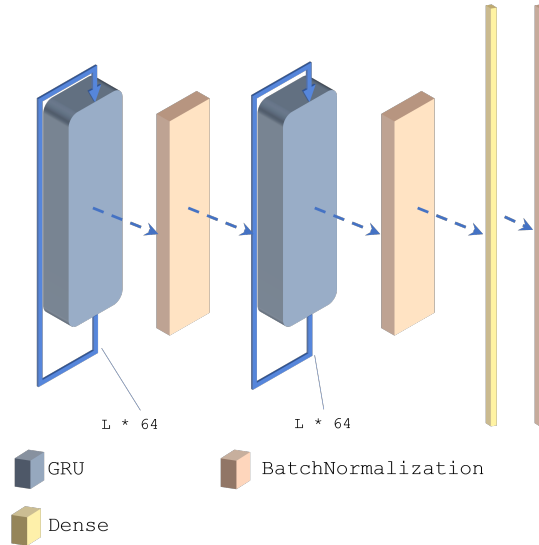
Figure 5.6: Embedding Architecture for EDA and PPG signals
