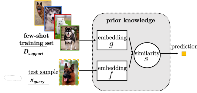
Figure 2.12: Schematic of Distance Metric Learning Methods
