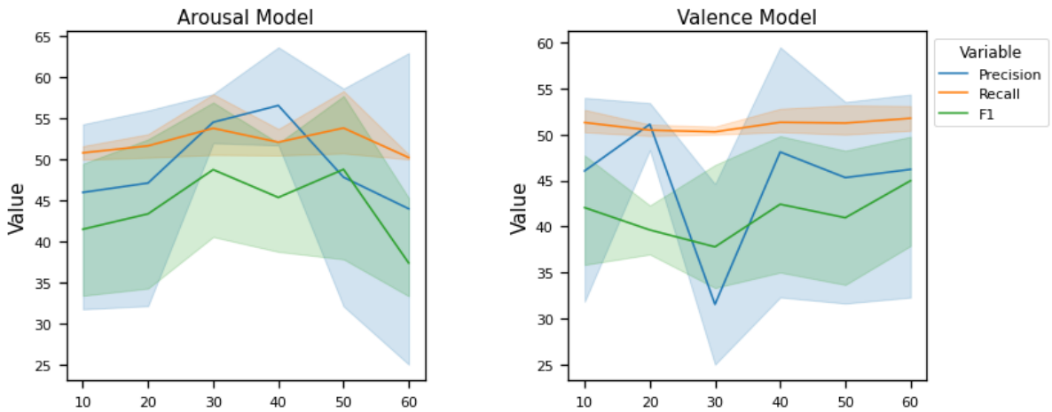
Figure 6.15: RECOLA : Distribution of Query Set Precision ( P ), Recall ( R ) and F1 Score ( F1 ) for different cases
