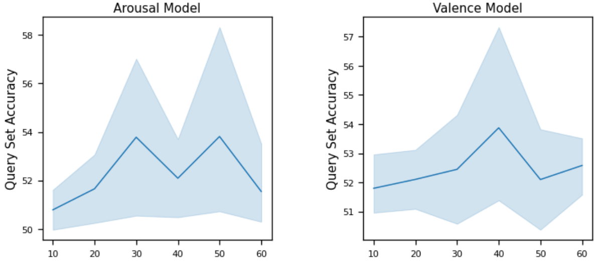
Figure 6.14: RECOLA : Distribution of Query Set Binary Accuracy ( A_q ) for different cases
