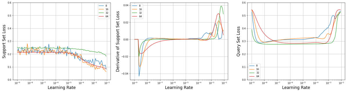
Figure 6.2: K-EmoCon : Learning-rate Range Test for Arousal Model
