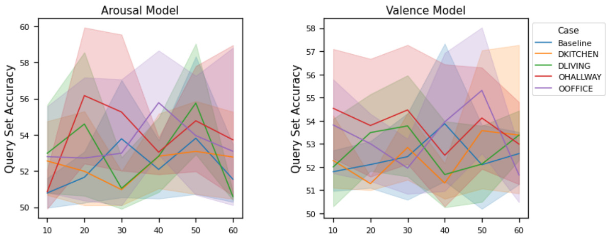
Figure 6.17: RECOLA : Summary of Query Set Binary Accuracy ( A_q ) for different cases
