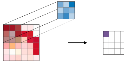
Figure 2.5: Convolutional Layer
