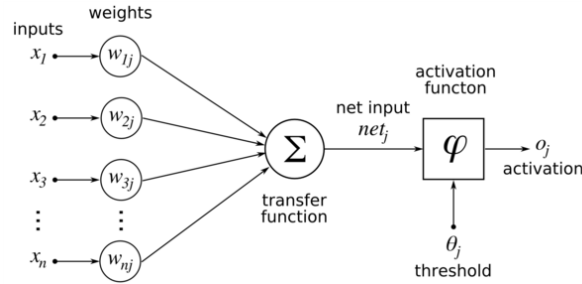
Figure 2.2: Perceptron
