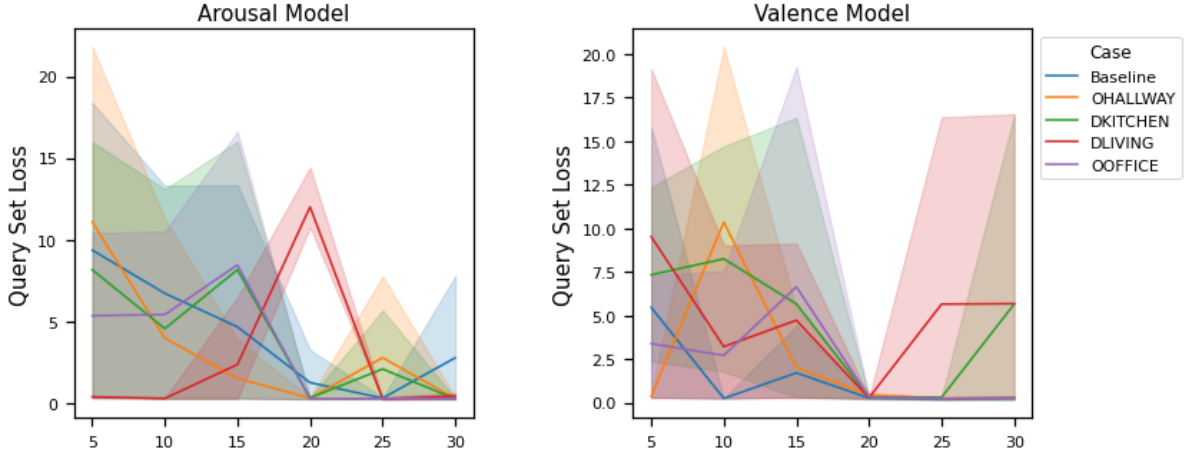
Figure 6.7: K-EmoCon : Summary of Query Set Contrastive Loss ( L_q ) for different cases
