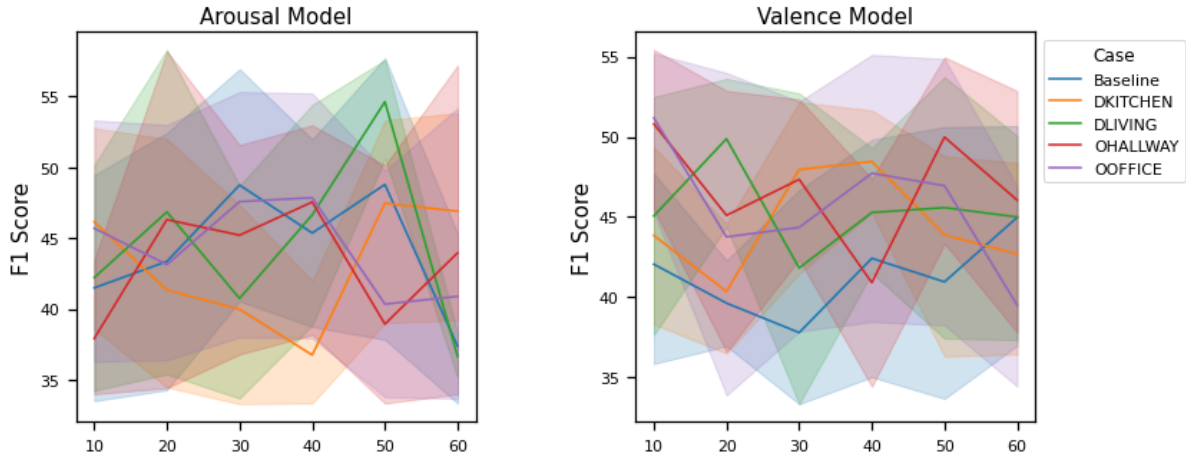
Figure 6.18: RECOLA : Summary of Query Set F1 Score ( F1 ) for different cases
