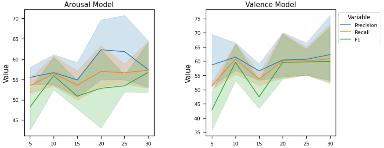
Figure 6.6: K-EmoCon : Distribution of Query set Precision ( P ), Recall ( R ) and F1 Score ( F1 ) for Baseline Model
