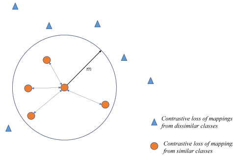
Figure 5.7: Illustration of Contrastive Loss and margin between samples
