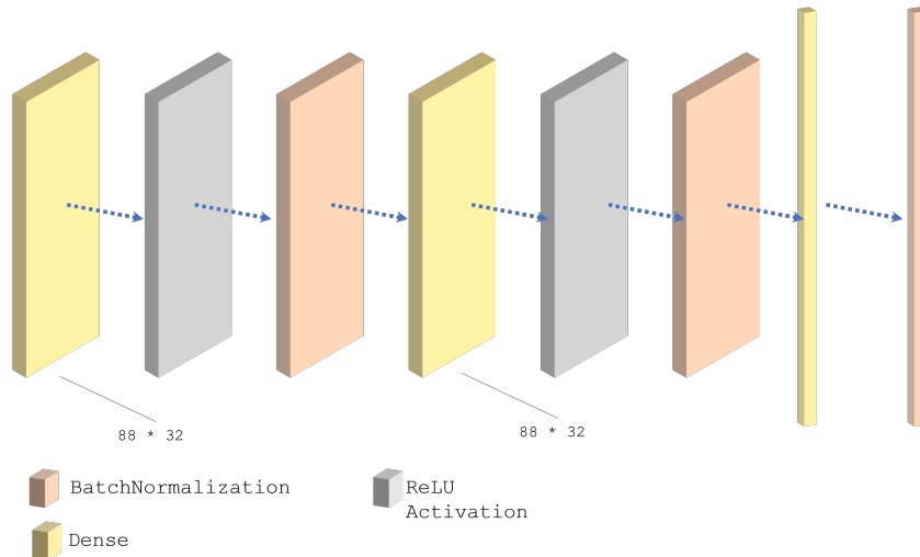
Figure 5.4: Embedding Architecture for eGeMAPS
