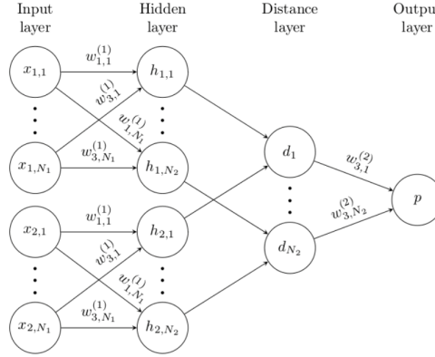
Figure 5.2: Siamese Network Architecture [45]
