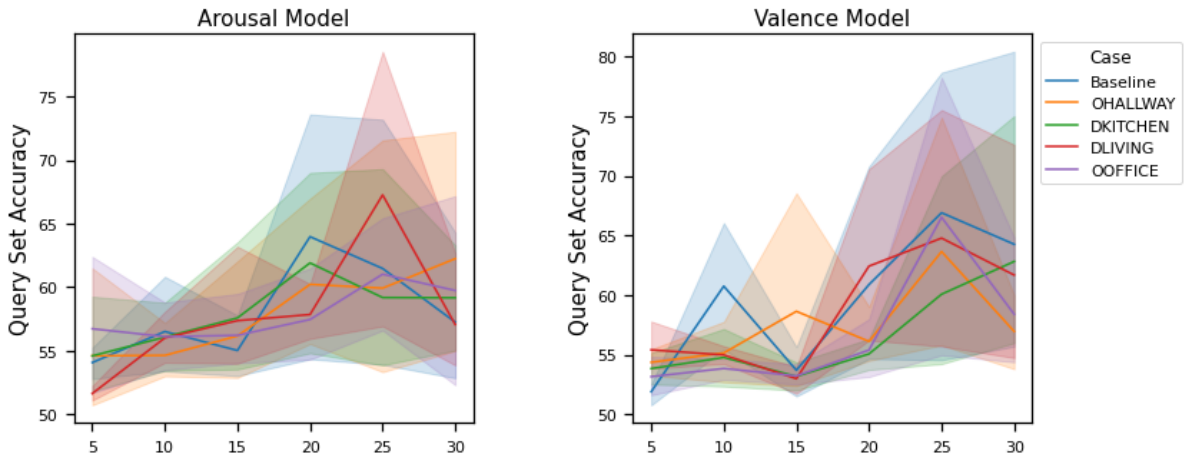
Figure 6.8: K-EmoCon : Summary of Query Set Binary Accuracy ( A_q ) for different cases
