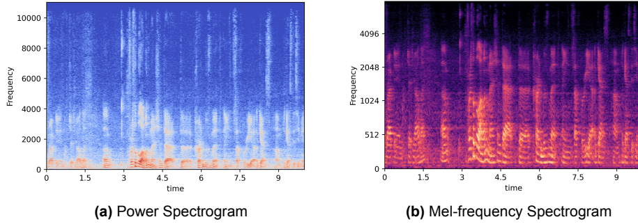
Figure 3.3: Comparison of Spectrograms
