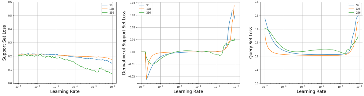
Figure 6.11: RECOLA : Learning rate Range Test Contrastive Loss for Arousal Model
