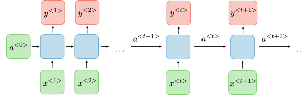
Figure 2.8: Recurrent Neural Network
