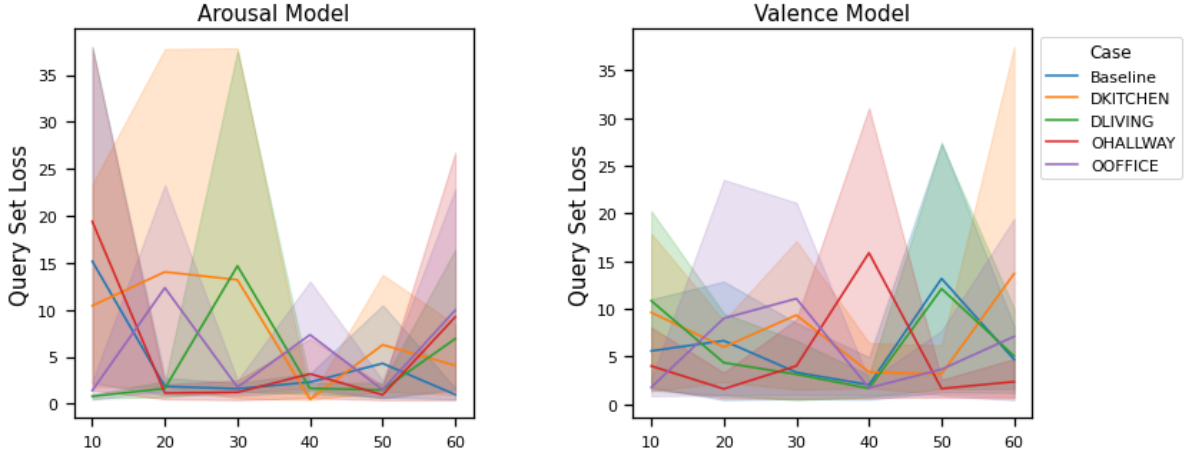
Figure 6.16: RECOLA : Summary of Query Set Contrastive Loss ( L_q ) for different cases
