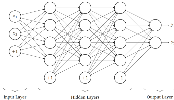
Figure 2.3: Deep Neural Network (Multilayer Perceptron)
