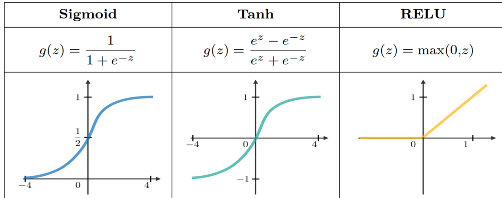
Figure 2.4: Activation Layers
