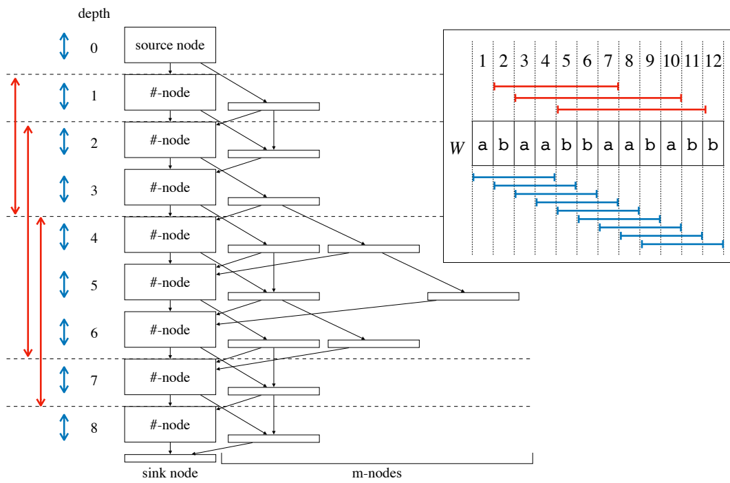
Figure 3 The decision DAG for W = \text{abaabbaababb} , k = 4 , and S = \{[2, 7], [3, 10], [5, 11]\} .
