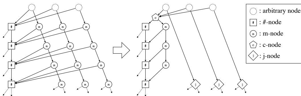
■ Figure 2 An example of contracting a part of the decision DAG. Before contracting, there are three parallel m-paths each of length 2^2 = 4 . We contract each m-path to a j-node corresponding to the case in which four consecutive non-sensitive patterns are merged. Also, we create an m-path of length 3 preceded by a c-node corresponding to the case in which at least one gadget is inserted.
