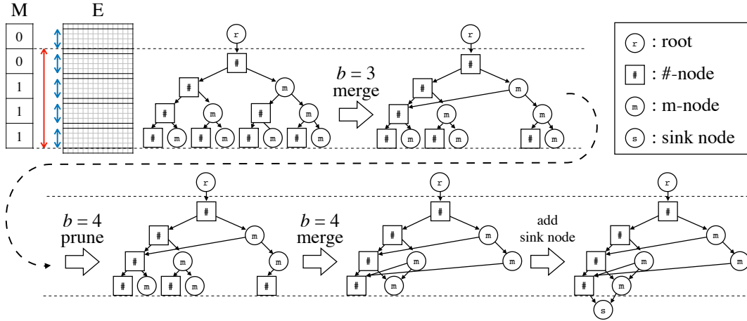
■ Figure 1 An example for pruning and merging a decision tree. The red arrow represents a long sensitive pattern, and blue arrows represent non-sensitive patterns. The tree on the top-left represents the decision tree after pruning or merging operations for depths b = 0, 1, 2 . For b = 3 , we merge two #-nodes by Rule 3. For b = 4 , we prune an m-node by Rule 2 since merging four non-sensitive patterns following the node results creating a sensitive pattern. Furthermore, we merge three #-nodes by Rule 3, and merge two m-nodes by Rule 4. Finally, we add the sink node at the bottom.
