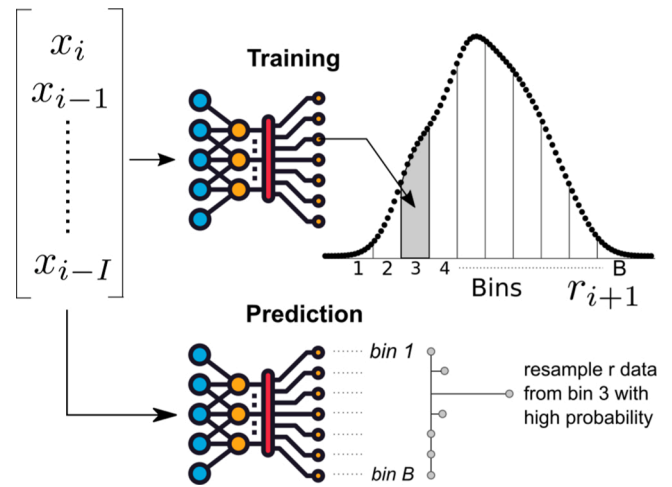
Fig. 9. A schematic depicting the QSN training and prediction.
