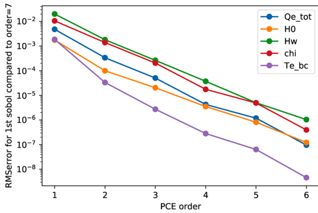
Fig. 8. The convergence of the predicted mean and standard deviation (top) and Sobol first indices (bottom) with increasing order of the PCE expansion.
