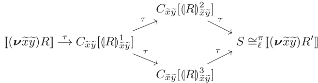
Fig. 11 Elements in the set of intermediate redexes (cf. Notation 14)
