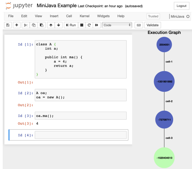
Figure 3: Notebook example.
