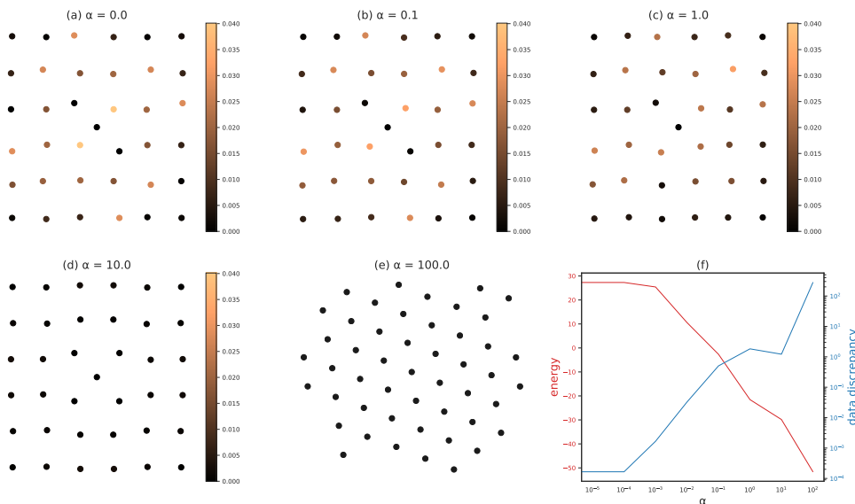
Fig. 5. (a)-(d): Increasing the weighting of the energy term from \alpha = 0.0 to \alpha = 10.0 helps to resolve the correct atomic configuration. The reconstructed atoms are coloured according to their Euclidean distance from the atoms in the ground truth. (e) At high values of \alpha , the reconstructions have a high data discrepancy and correspond to one of the global minima of the potential energy. (f) From the plots of potential energy and data discrepancy, an optimal value of \alpha can be selected.
