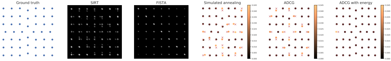
Fig. 4. Reconstructions of a vacancy defect from three projections. For the simulated annealing, ADCG and ADCG with energy reconstructions, atoms are coloured according to their Euclidean distance from the ground truth. Ground truth positions are marked with red crosses.
