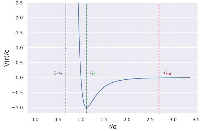
Fig. 2. The normalised Lennard-Jones pair potential as a function of normalised interatomic separation.
