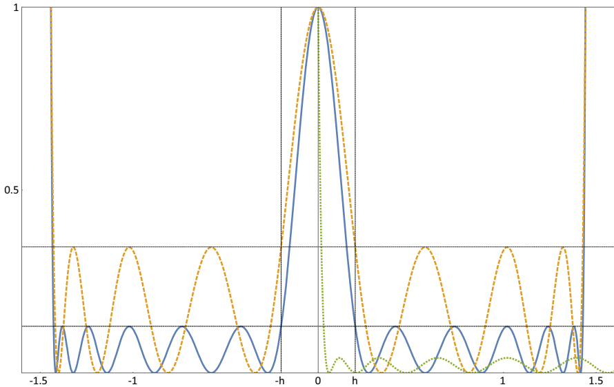
Fig. 5 The needle polynomials v_4^h (dashed), v_6^h (solid) and the \frac{1}{2} -needle \widehat{v}_4^h (dotted) for h = 1/5
