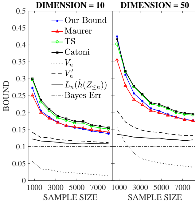
Figure 2: Results for the synthetic data with informed priors.
