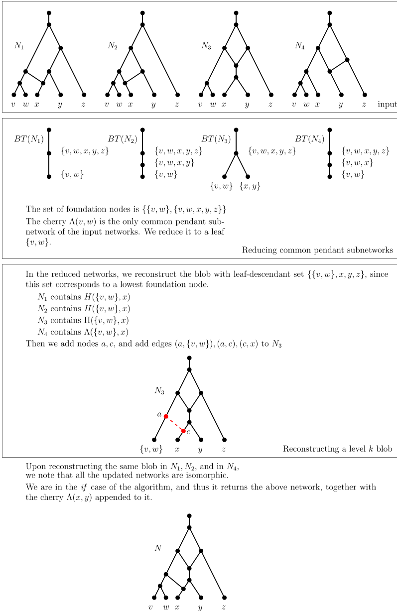
Fig. 16 (Color figure online) An example of the algorithm TCMLLS-RECONSTRUCTION( \{N_1, N_2, N_3, N_4\} ). Initially, the common pendant subnetworks of the four input networks are determined by looking at their blob trees. In this case, this is the cherry \Lambda(v, w) (line 1). Upon reducing the cherry \Lambda(v, w) to a leaf \{v, w\} in all the MLLSs, the lowest foundation node is found to be \{\{v, w\}, x, y, z\} . We find a leaf pair \{v, w\} in all the MLLSs, the lowest foundation node is found to be \{\{v, w\}, x\} specified in line 4 of the algorithm. Since N_3 contains \Pi(\{v, w\}, x) , we reconstruct this blob in N_3 , shown by the red dashed edge (line 5). After reconstructing the same blob in all the other networks N_1, N_2 and N_4 , we see that the networks are all isomorphic (we enter the if statement of line 12). The algorithm then returns the network N
