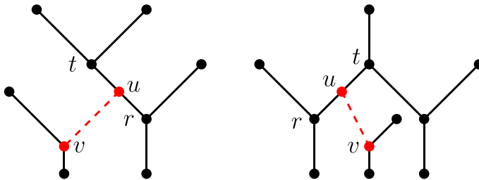
Fig. 4 (Color figure online) Visual aid for the proof of Lemma 3. The left case is when N' contains a reticulation t that is a parent of a reticulation r . The right case is when a tree node t is a parent of two reticulations. In either case, the red dashed edge (u, v) must be inserted in these particular places to obtain N , and in either case N is not tree-child
