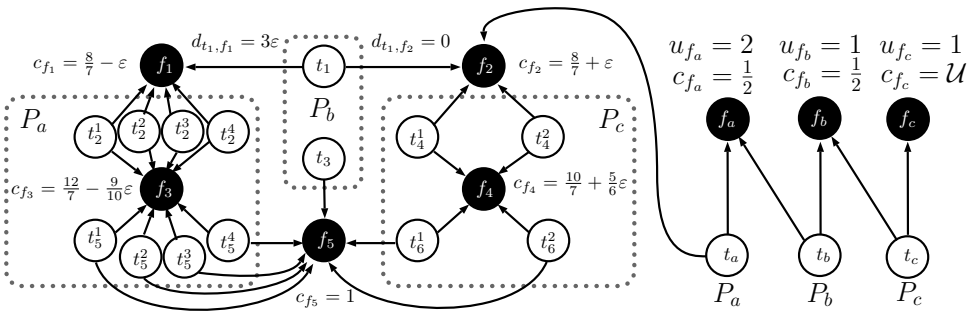
Fig. 6. An instance of capacitated FLG-FC with unbounded PoS. All connections have zero cost (except d_{t_1, f_1} , which has cost 3\epsilon ). Any facility f without a capacity restriction indicated is unlimited, i.e., u_f \geq 8 . Labels next to terminals indicate which player controls the terminal.
